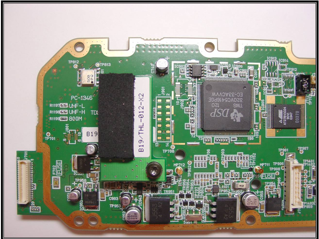
PHOTOGRAPH 7: AUDIO LOGIC BOARD COMPONENT SIDE – LEFT
