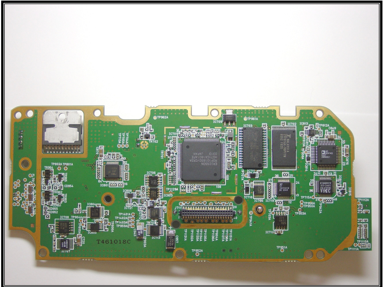
PHOTOGRAPH 6: AUDIO LOGIC BOARD SOLDER SIDE COMPLETE VIEW
