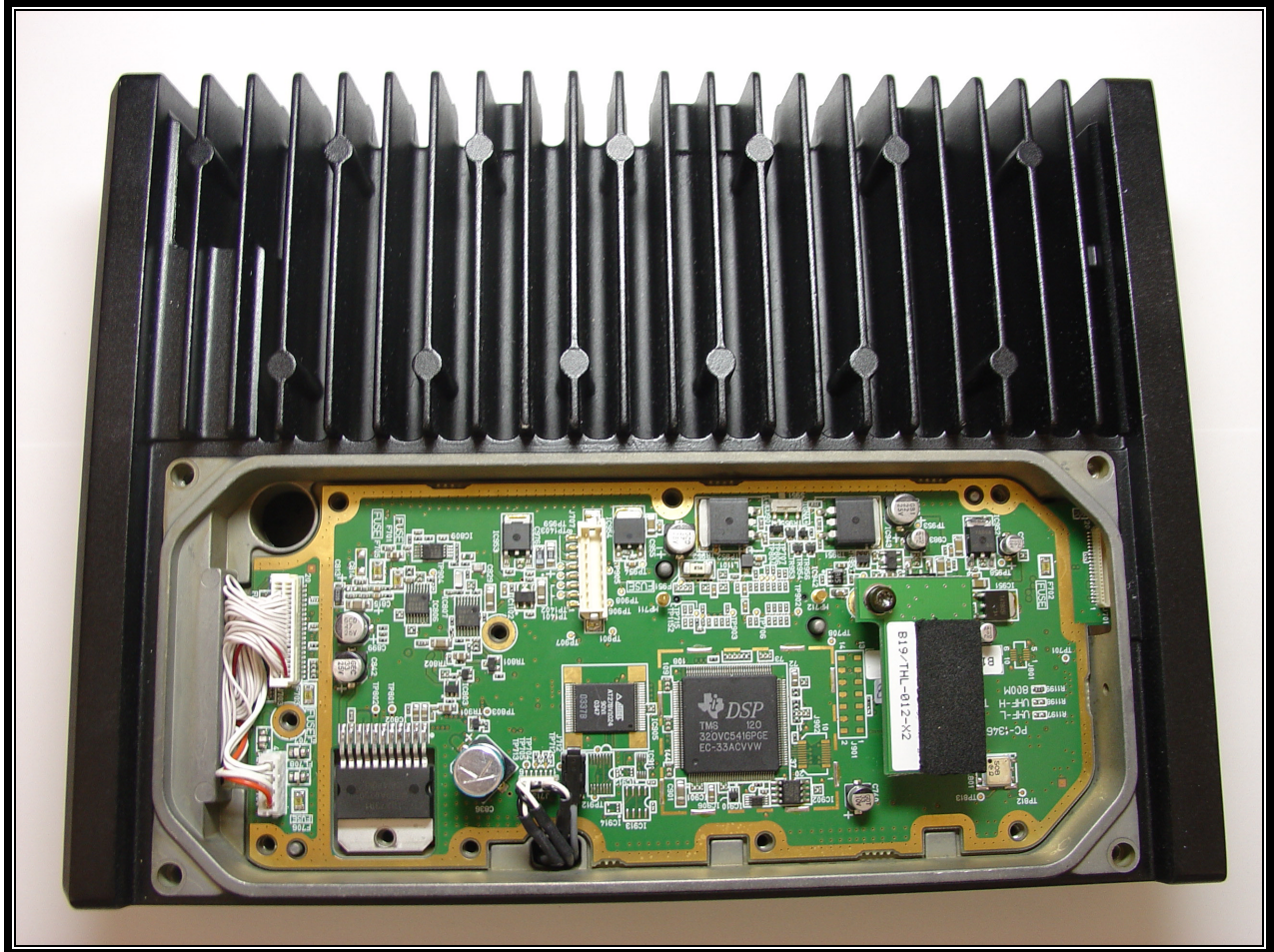
PHOTOGRAPH 4: TOP COVER AND INNER SHIELD REMOVED
