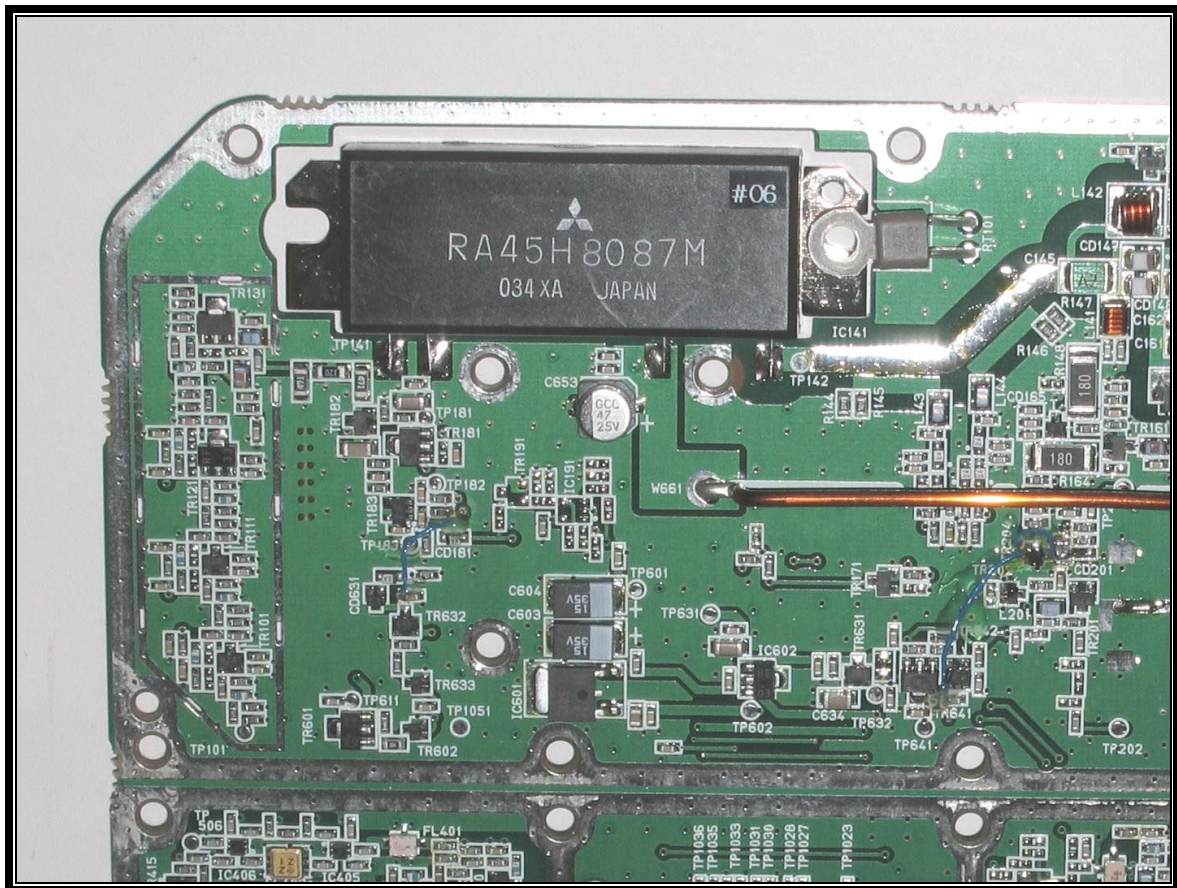
PHOTOGRAPH 21: TRX SYN BOARD COMPONENT SIDE, UPPER LEFT
