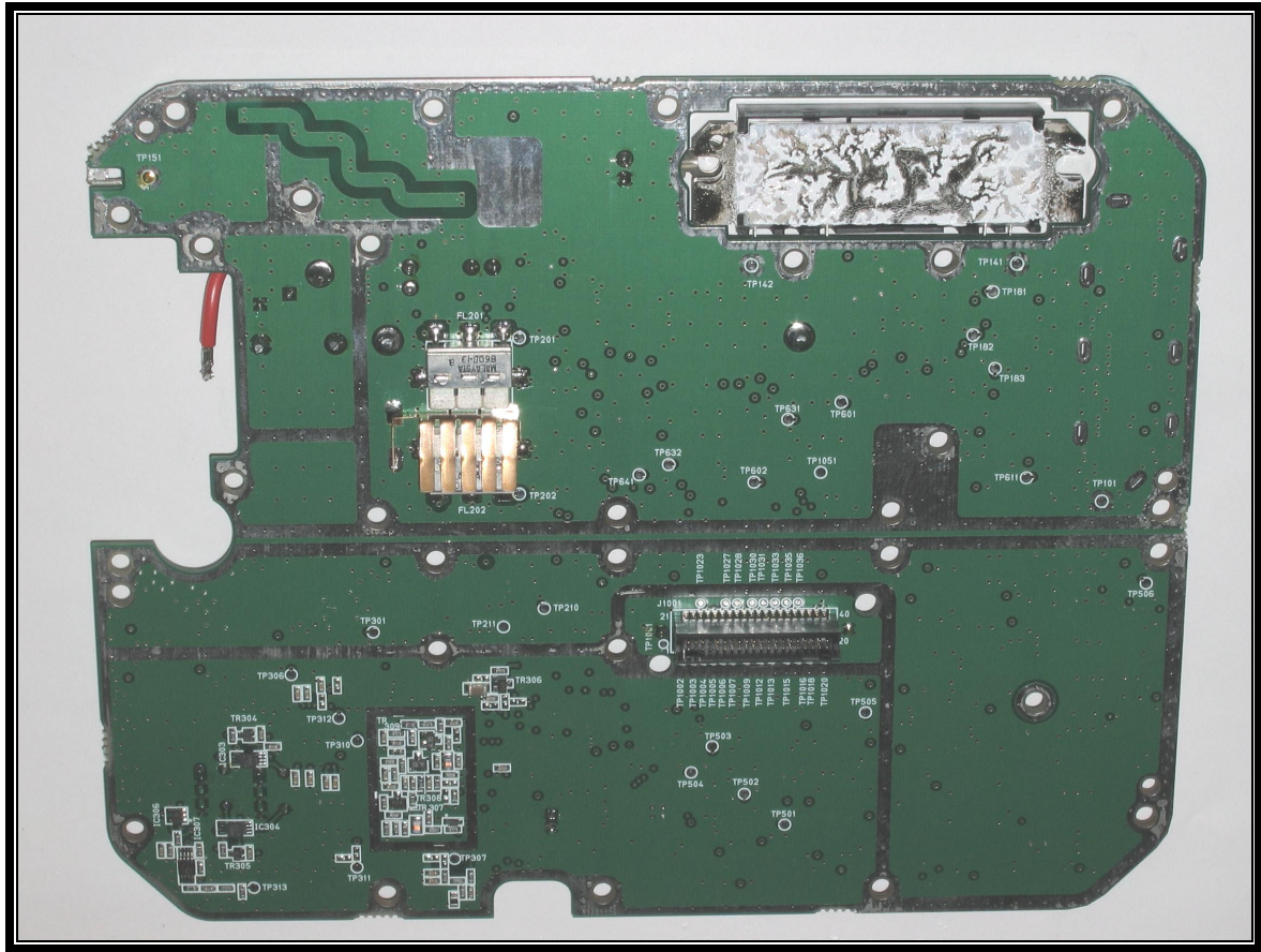
PHOTOGRAPH 23: TRX SYN BOARD SOLDER SIDE, COMPLETE VIEW
