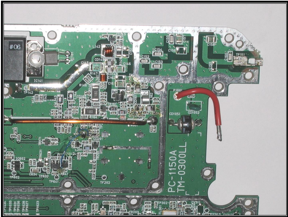
PHOTOGRAPH 22: TRX SYN BOARD COMPONENT SIDE, UPPER RIGH
