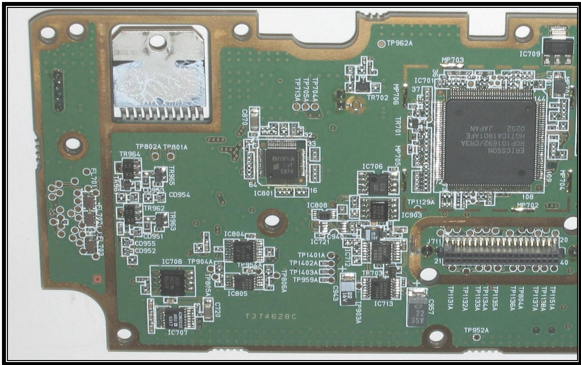
PHOTOGRAPH 15: AUDIO LOGIC BOARD SOLDER SIDE, LEFT SIDE
