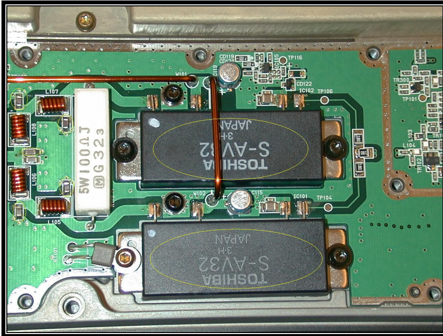
Photograph 6: TRX/SYNTHESIZER UNIT – CLOSE UP OF BOTH PA MODULES
