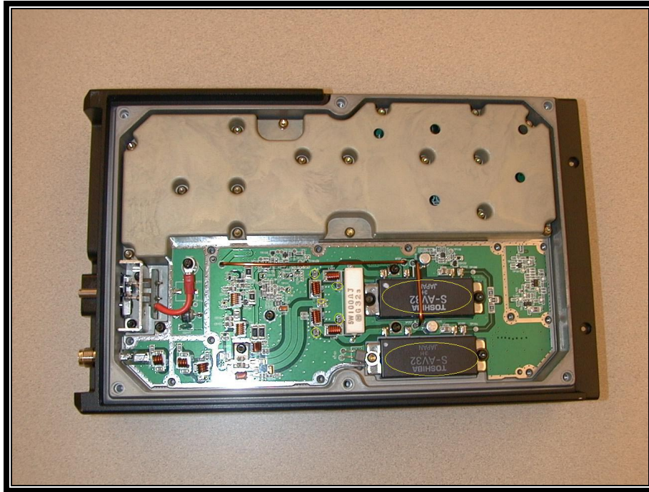
Photograph 5: TRX/SYNTHESIZER UNIT – VIEW OF BOARD
