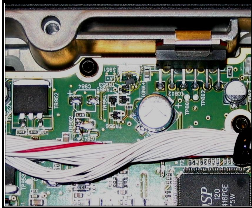
Photograph 4: AUDIO LOGIC BOARD – DETAILED VIEW OF POWER BLOCK
