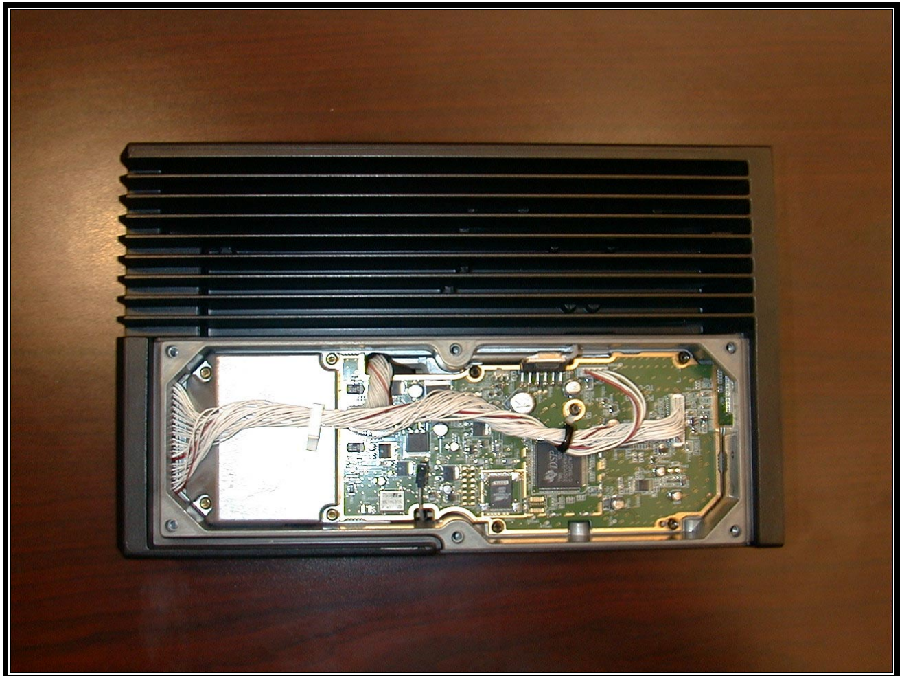
PHOTOGRAPH 10: AUDIO LOGIC BOARD INSTALLED
