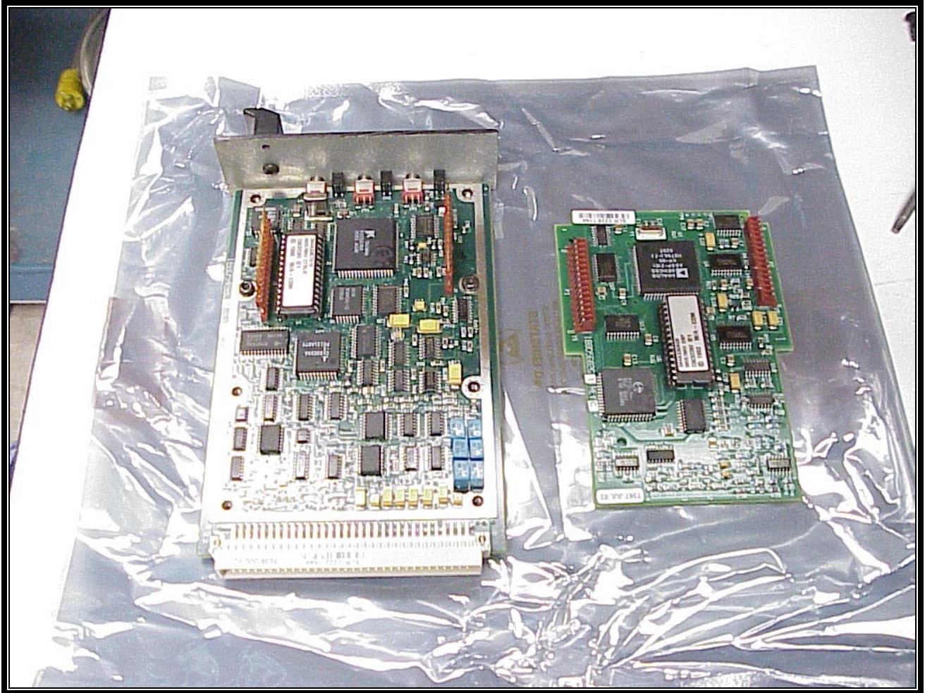
PHOTOGRAPH 32: SYSTEM MODULE, DSP BOARD TOP
