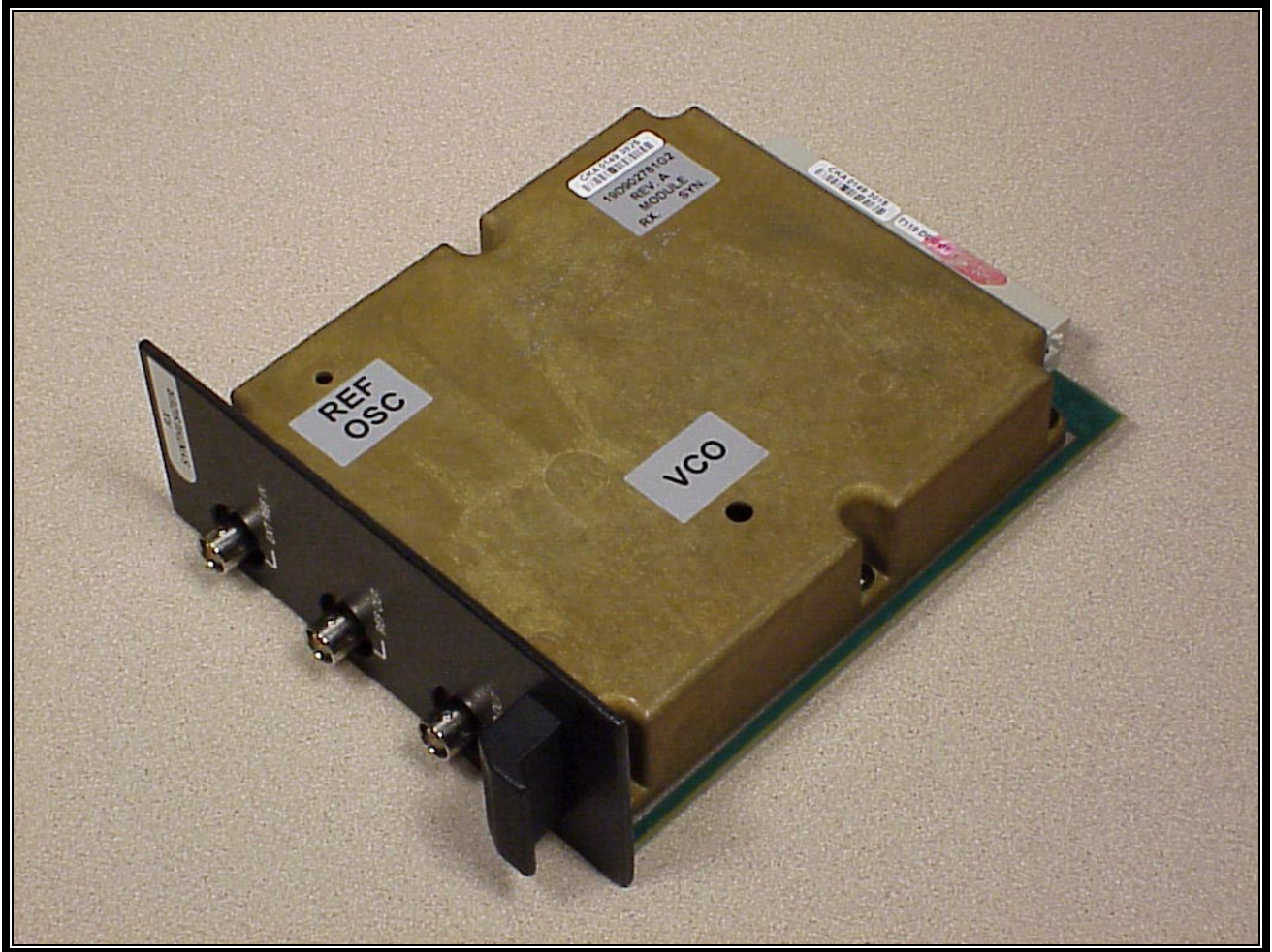
PHOTOGRAPH 43: RX SYNTH
