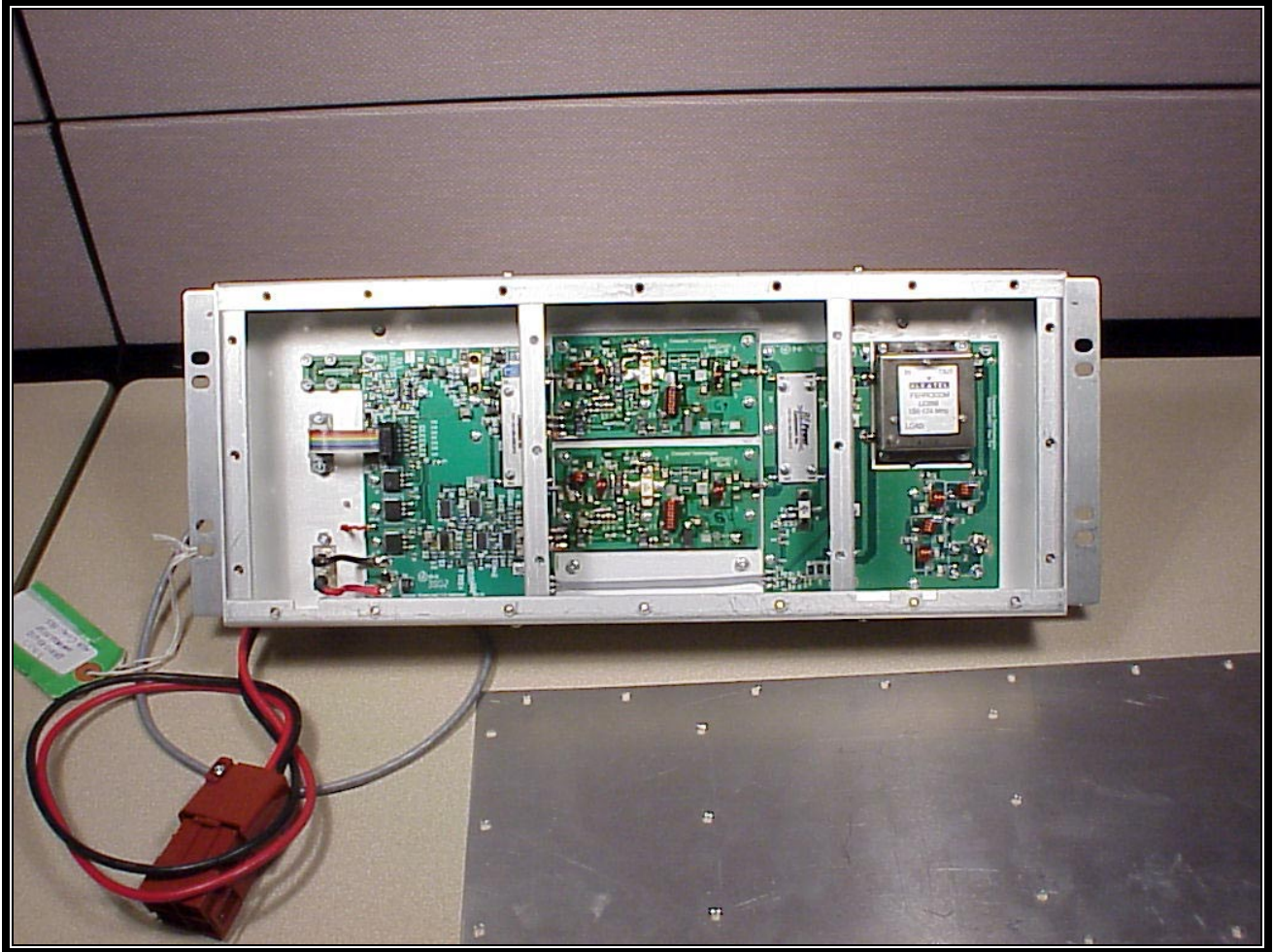
PHOTOGRAPH 13: VHF PA
