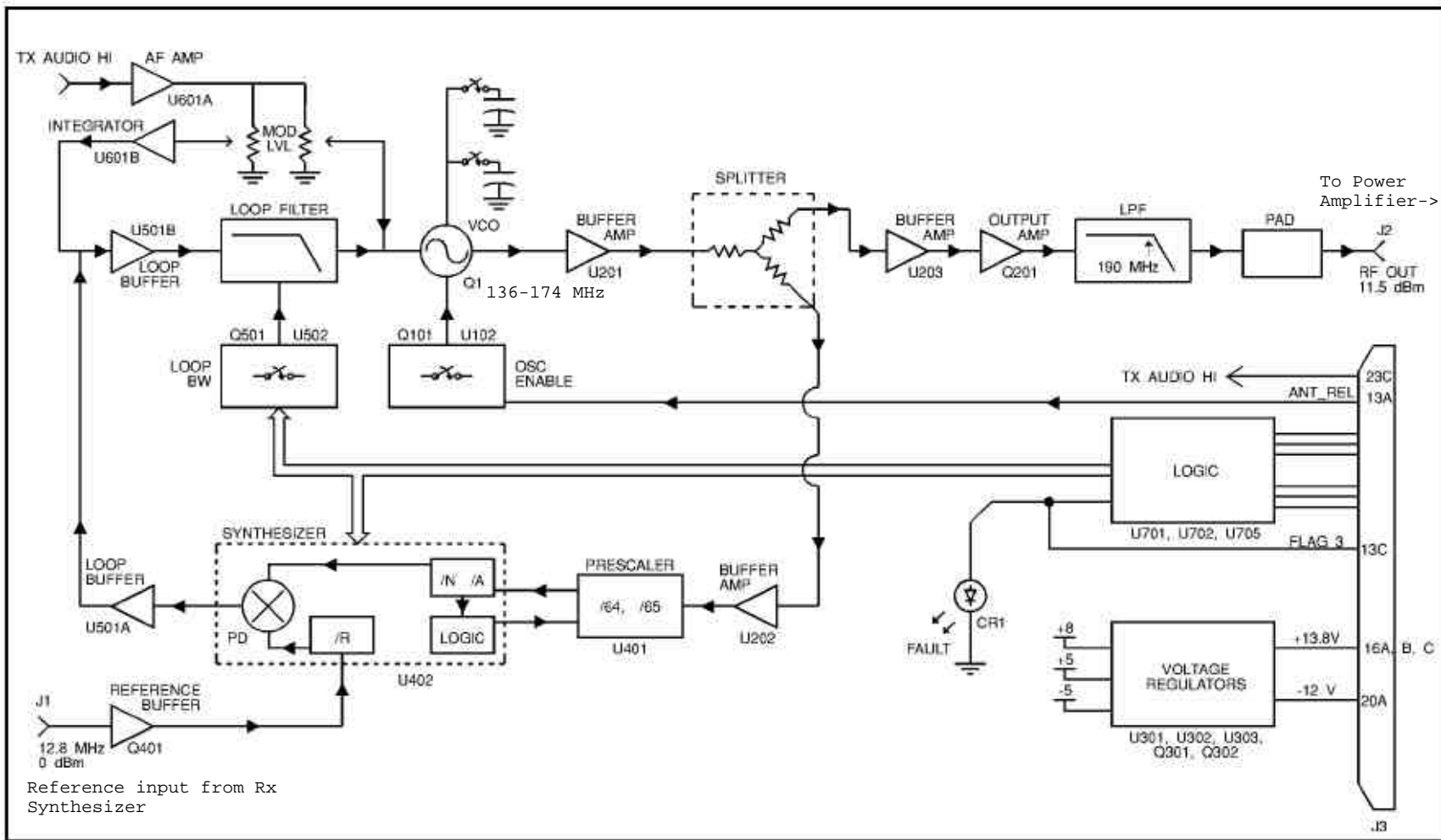
Figure 1 - Tx Synthesizer Block Diagram
