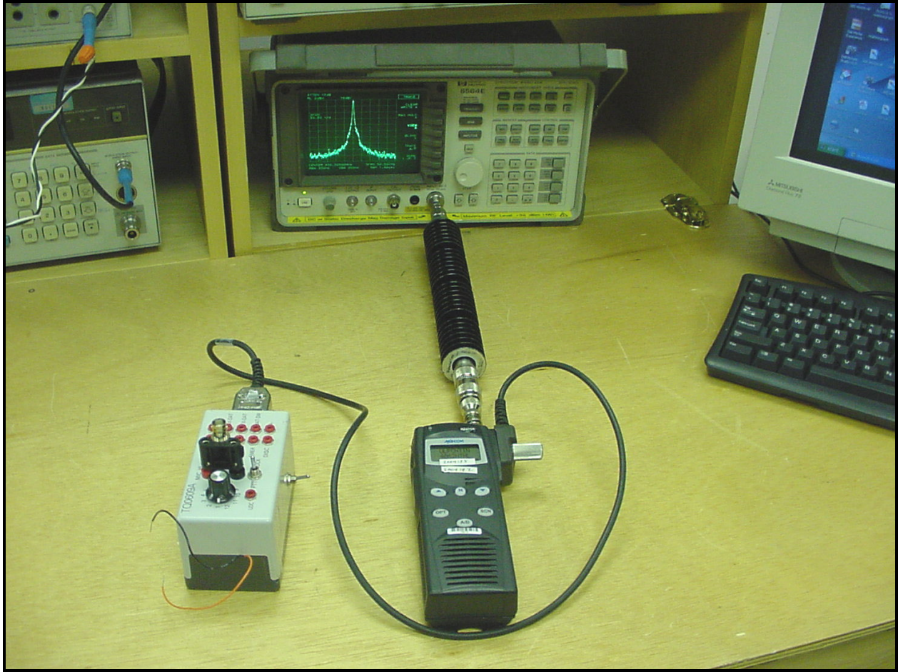
PHOTOGRAPH 6: CONDUCTED SPURIOUS/EMISSIONS MASKS MEASUREMENTS
