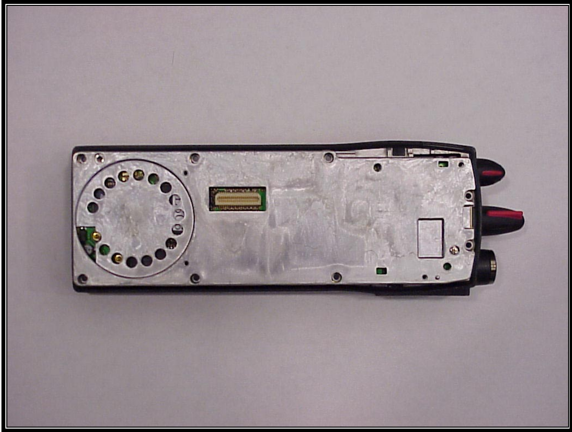
PHOTOGRAPH 12: UHF-L P7100 IP VIEW OF TOP OF RF SHIELD WITH INTERFACE BOARD REMOVED
