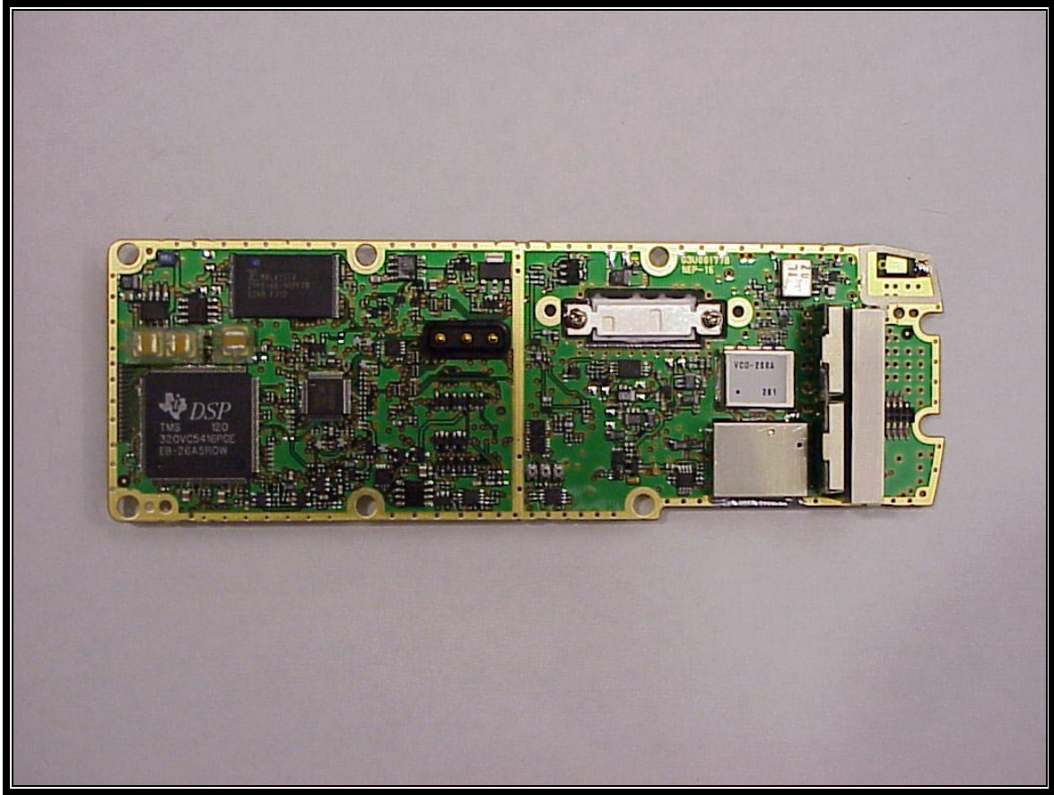
PHOTOGRAPH 14: UHF-L P7100 IP VIEW OF BOTTOM OF MAIN BOARD
