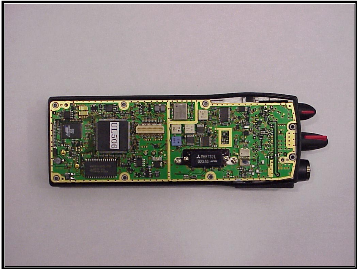
PHOTOGRAPH 13: UHF-L P7100 (IP) VIEW OF TOP OF MAIN BOARD WITH RF SHIELD REMOVED
