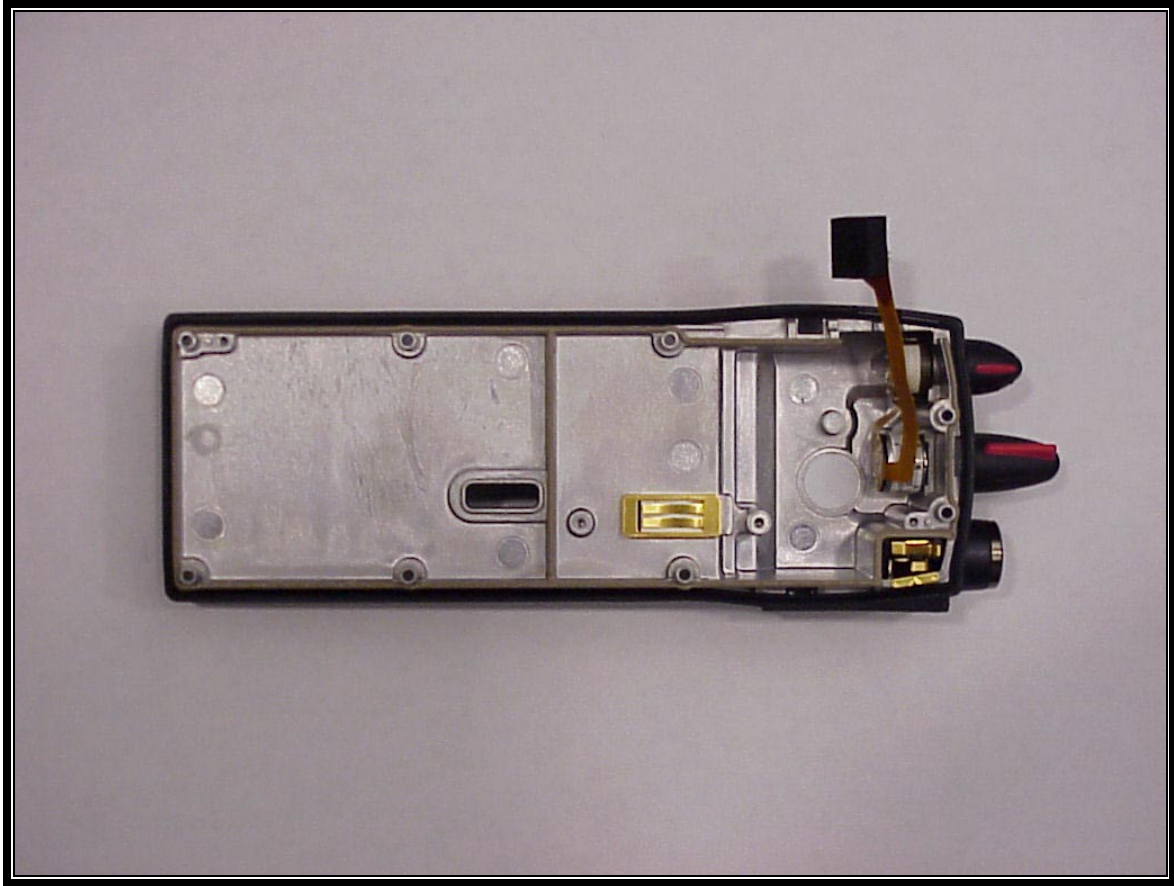
PHOTOGRAPH 15: UHF-L P7100 IP VIEW OF INSIDE WALL OF REAR CASTING WITH MAIN BOARD REMOVED
