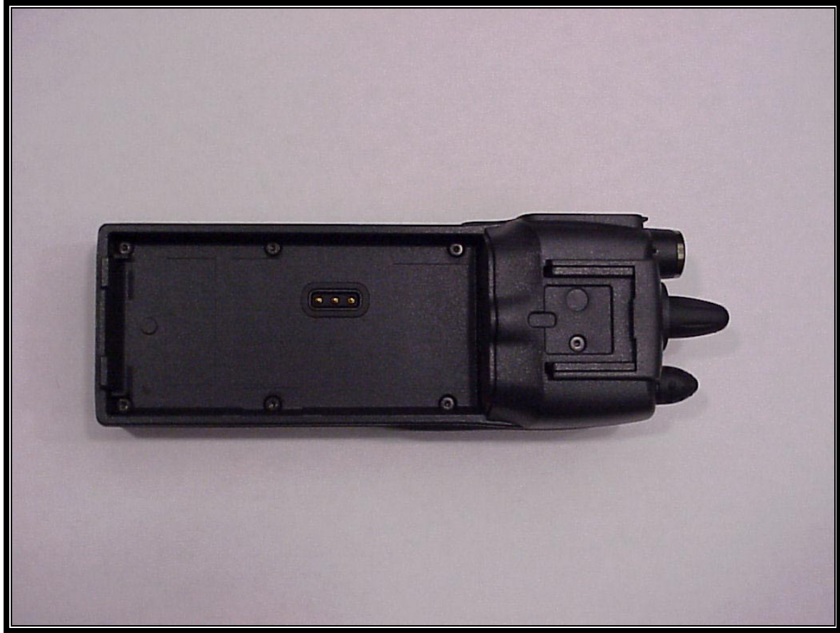
PHOTOGRAPH 7: UHF-L P7100 IP VIEW OF REAR CASTING
