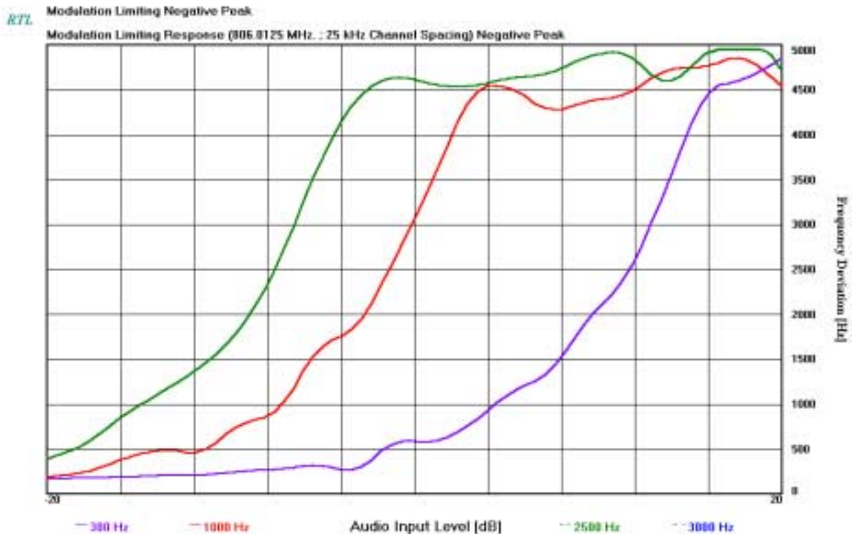
PLOT 11-1: MODULATION CHARACTERISTICS – MODULATION LIMITING: WIDE BAND NEGATIVE PEAK
