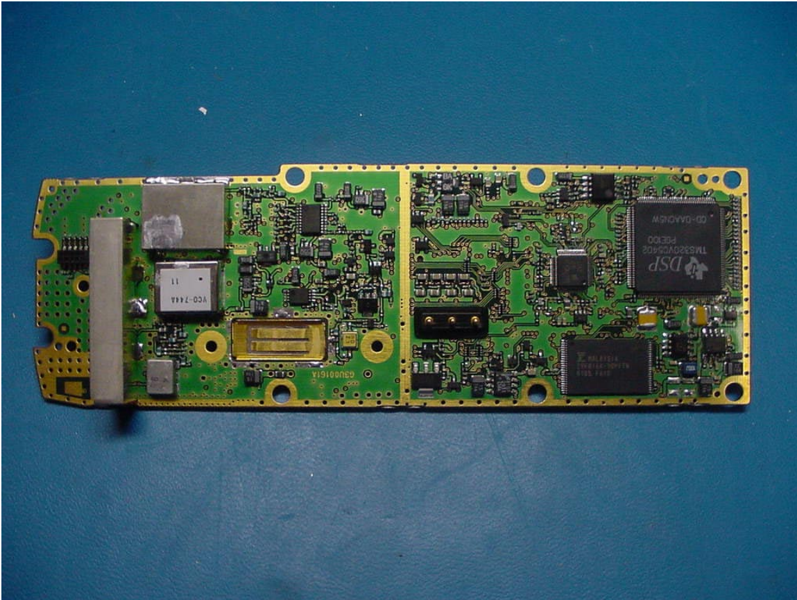
PHOTOGRAPH 15: BACK OF PCB WITH SHIELDS
