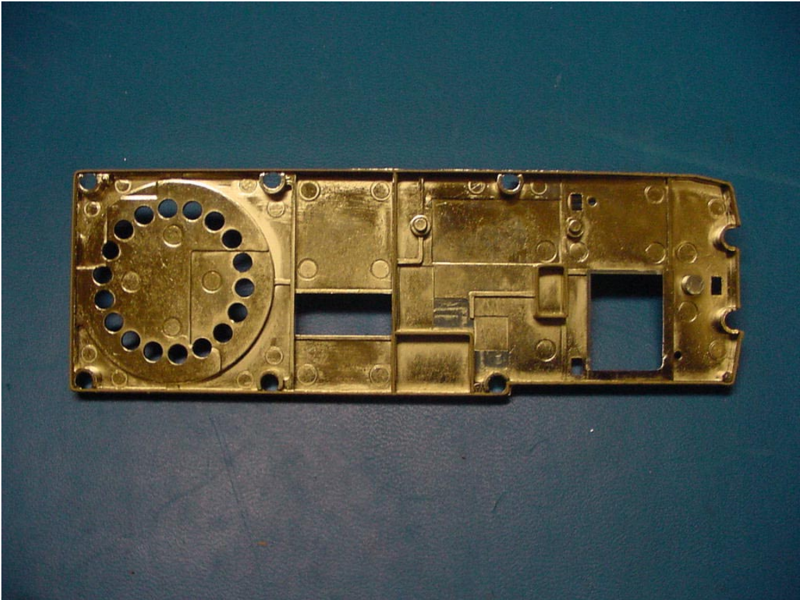
PHOTOGRAPH 20: REAR OF SHIELD
