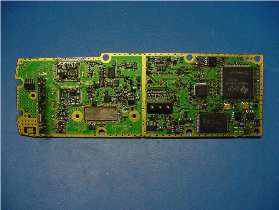
PHOTOGRAPH 14: FRONT OF PCB WITHOUT SHIELDS
