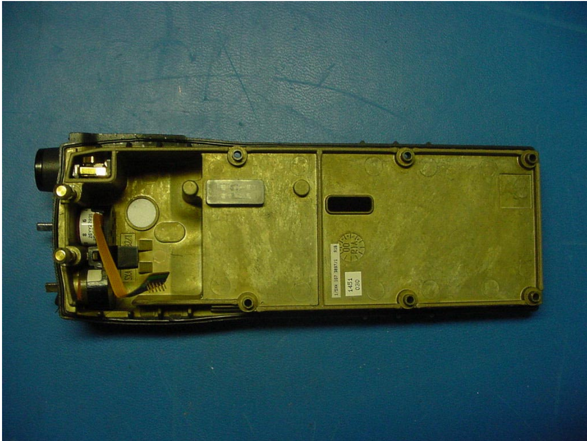
PHOTOGRAPH 16: INSIDE OF REAR CHASSIS
