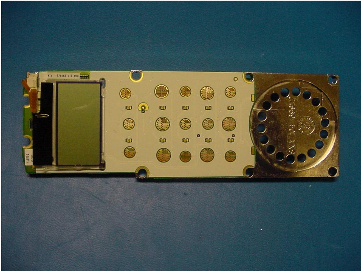
PHOTOGRAPH 18: FRONT OF SECONDARY PCB WITH LCD
