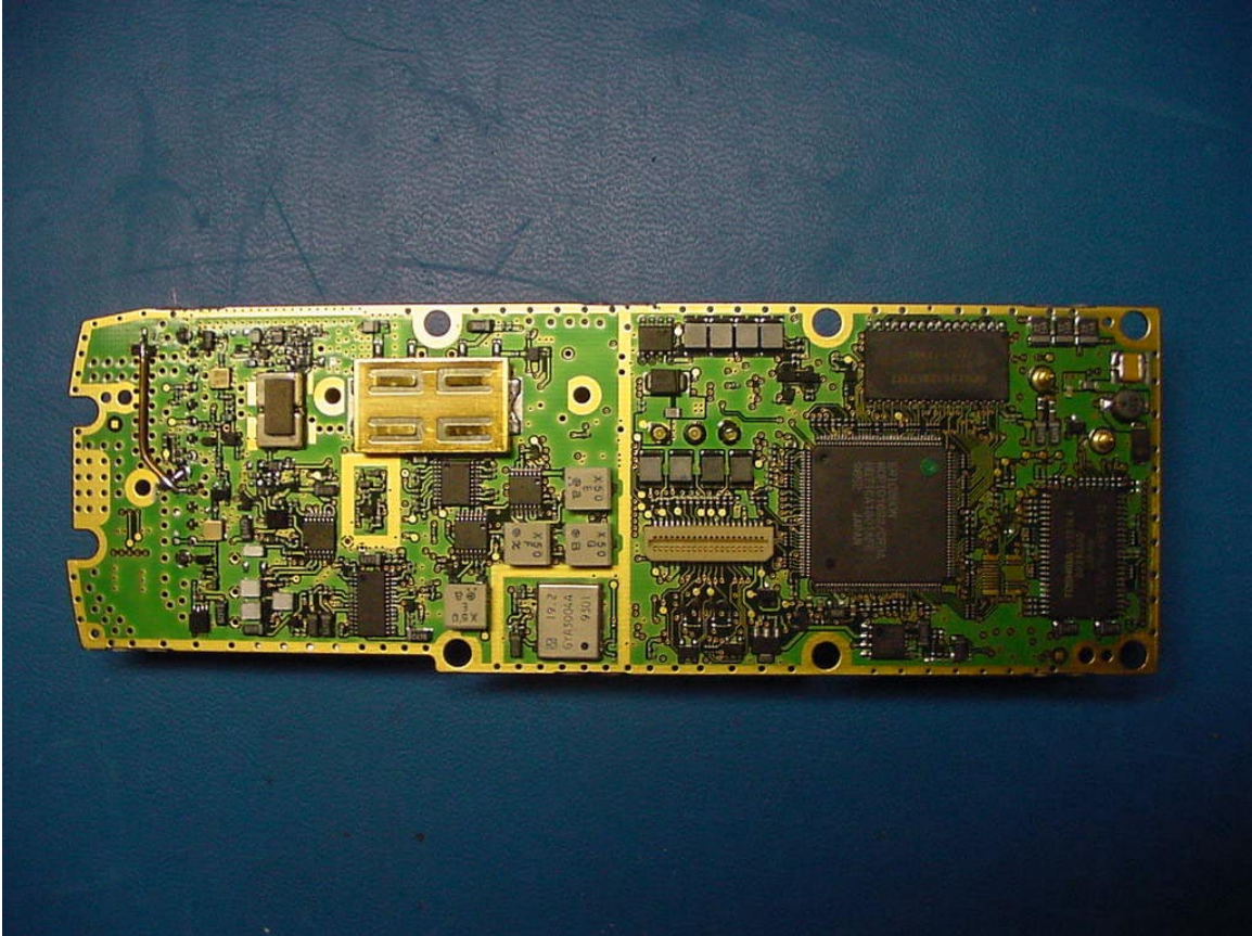
PHOTOGRAPH 13: FRONT OF PCB WITH SHIELDS
