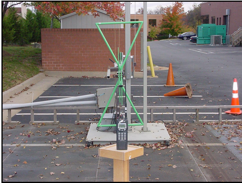
Photograph 5: Radiated Emissions Front View
