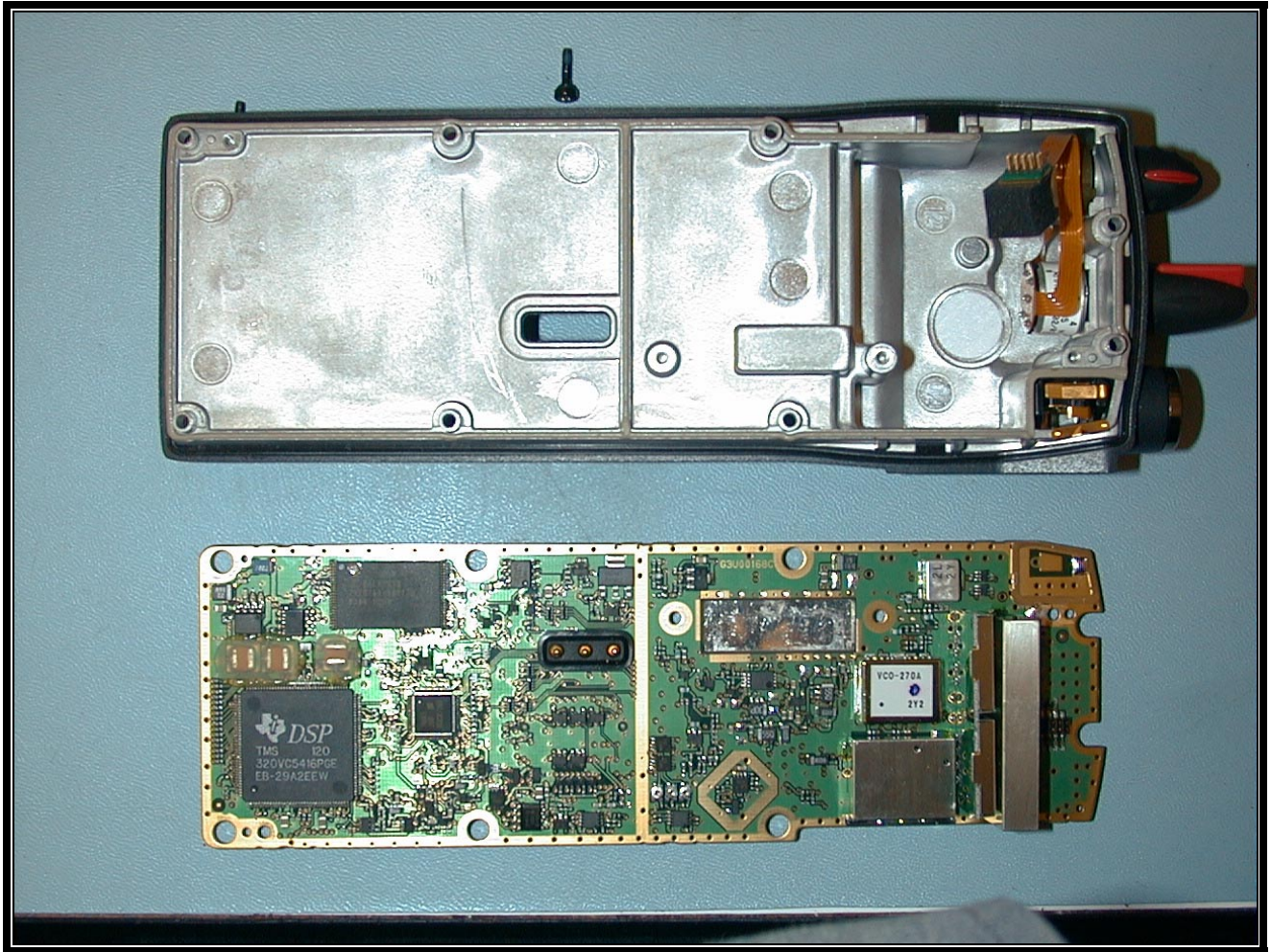
Photograph 2: Full View of New R1B Casting and Board
