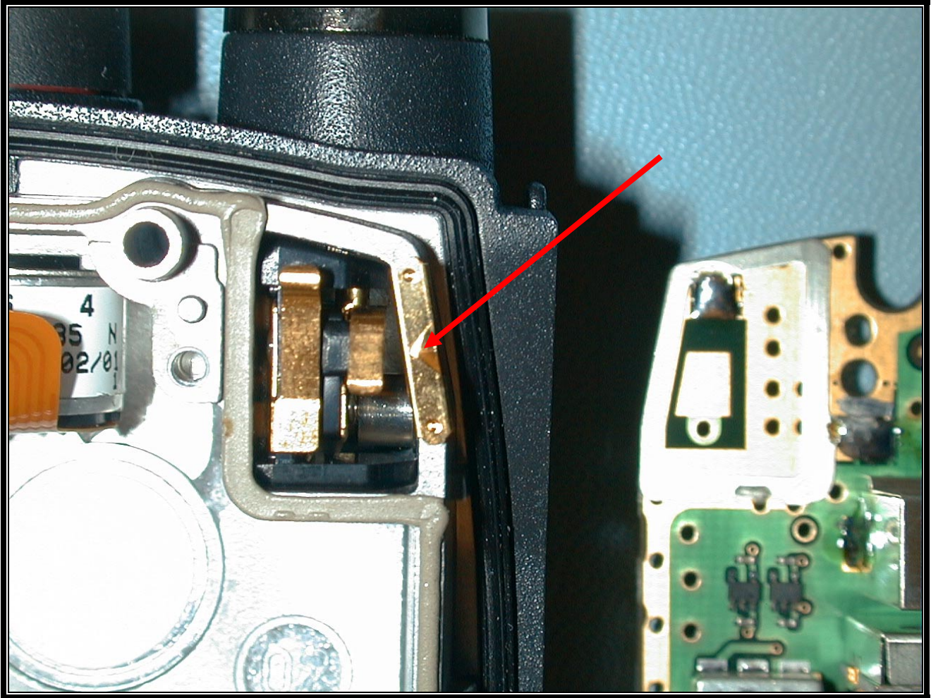
Photograph 4: Close-up of New R1B Antenna Launch Area
