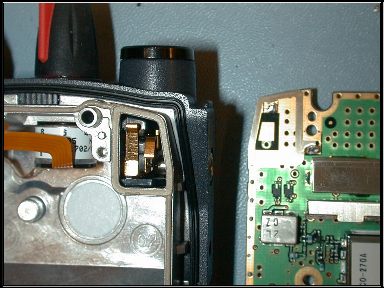
Photograph 3: Close-up of Original R1A Antenna Launch Area
