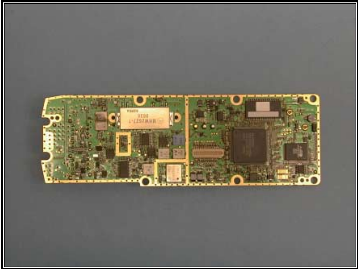
PHOTOGRAPH 5: FRONT SIDE OF MAIN BOARD
