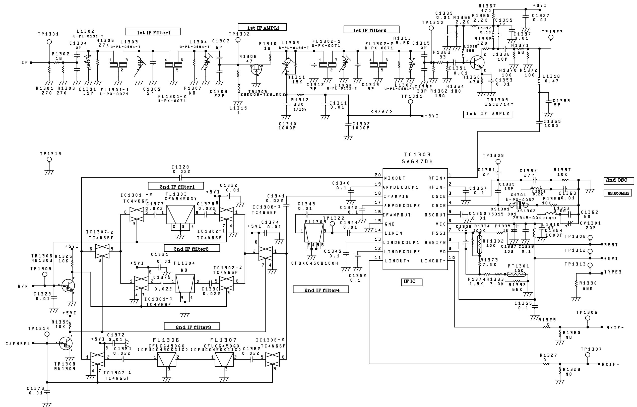
Schematic of JAGUAR 700M(800MHz) A/L&IF Unit
