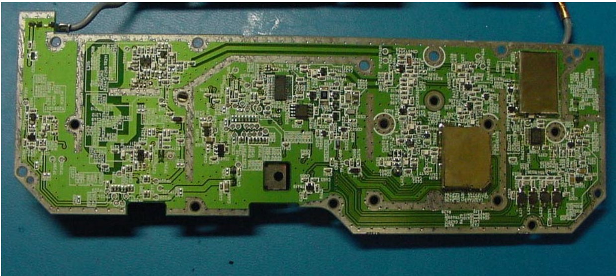
PHOTOGRAPH 15: PCB A REAR WITH SHIELDS
