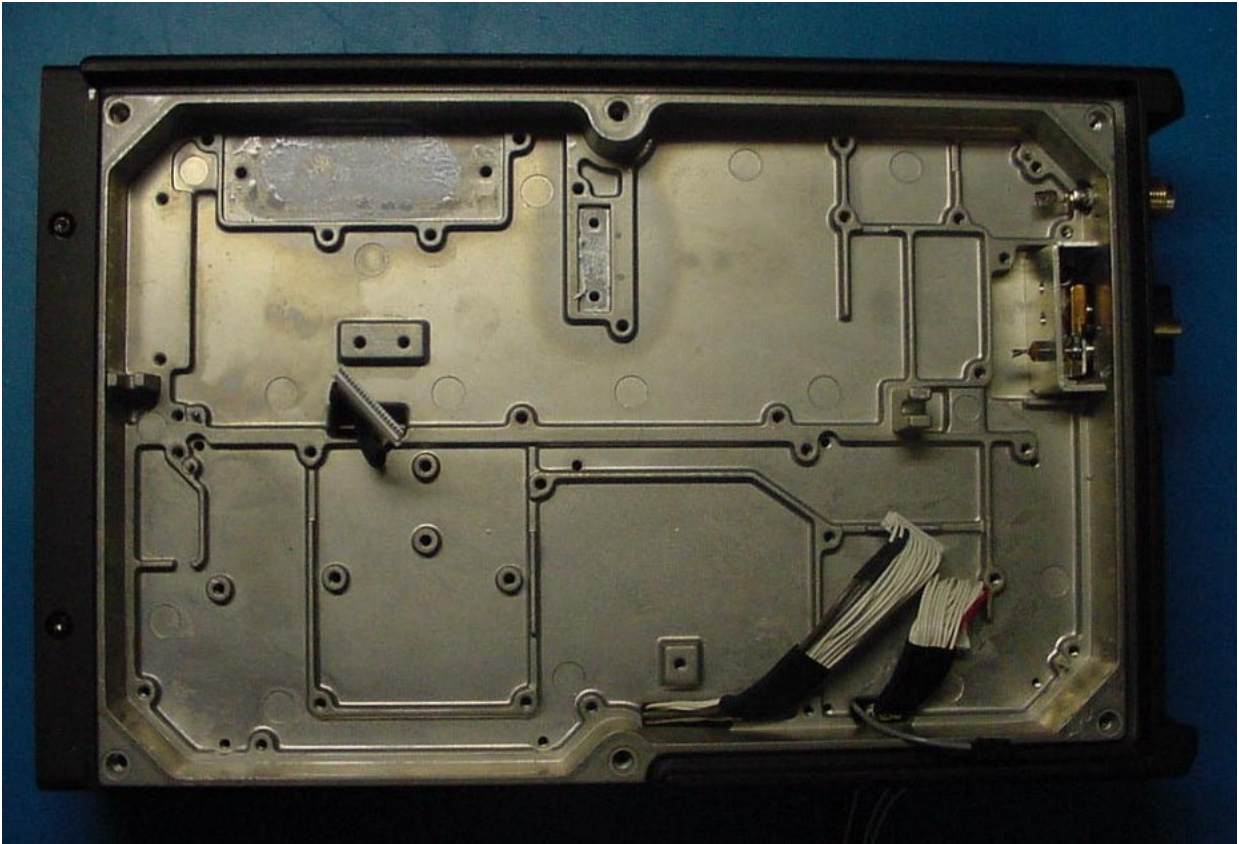
PHOTOGRAPH 21: BOTTOM INSIDE CASE
