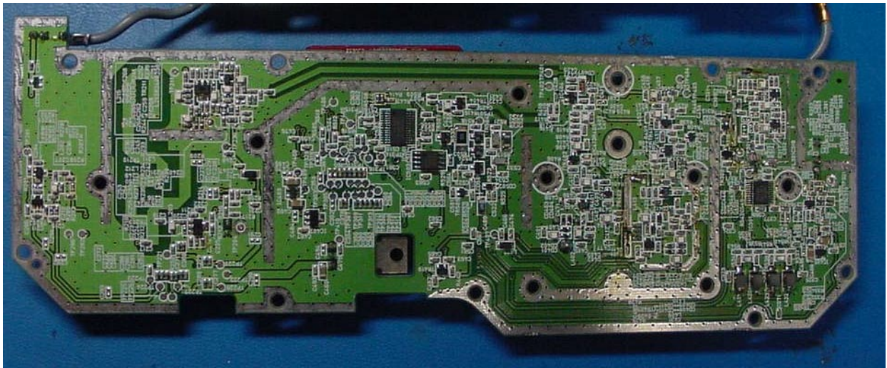
PHOTOGRAPH 16: PCB A REAR WITHOUT SHIELDS
