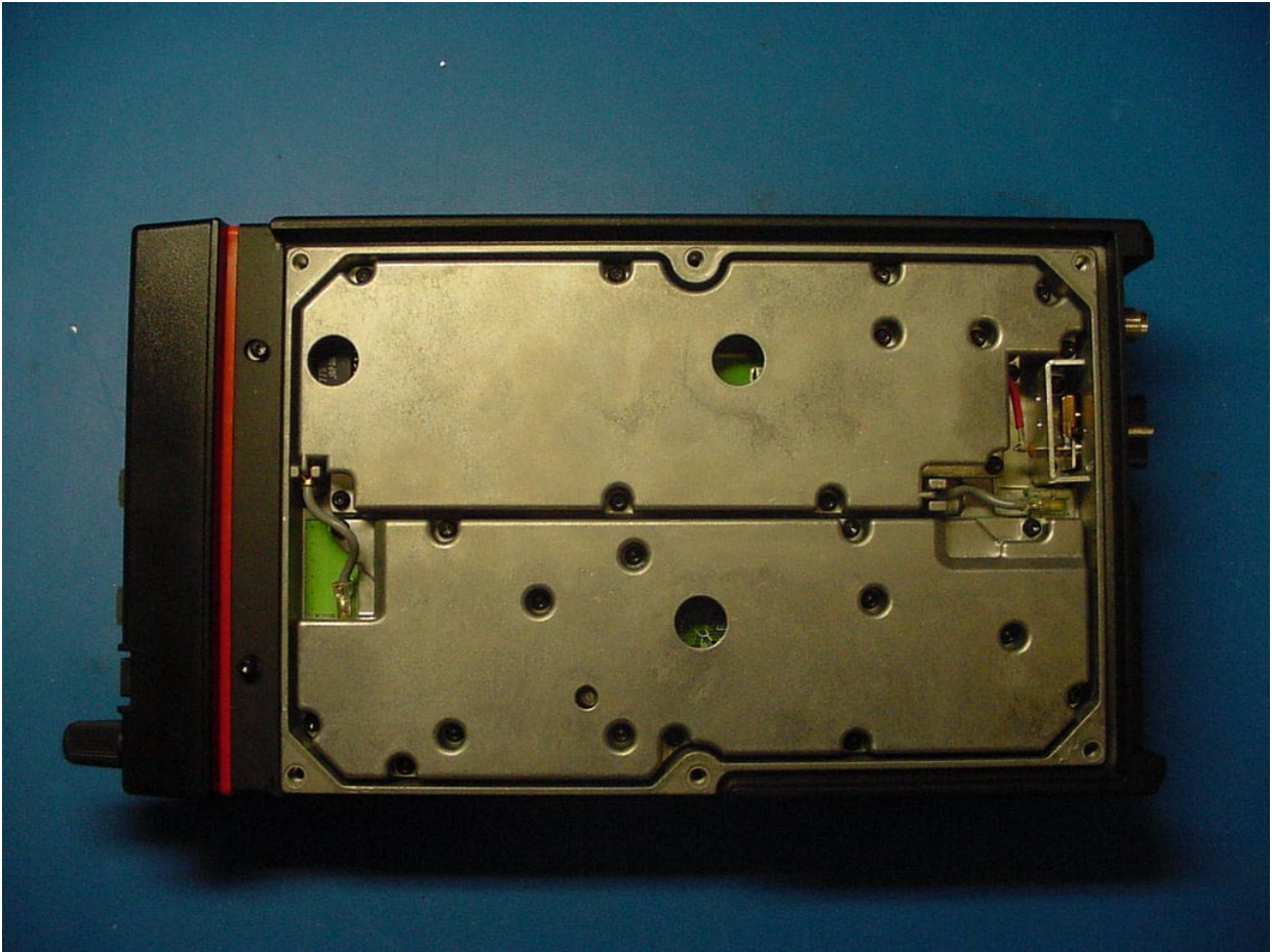
PHOTOGRAPH 22: BOTTOM WITH COVERS
