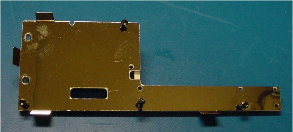
PHOTOGRAPH 36: SHIELD FRONT
