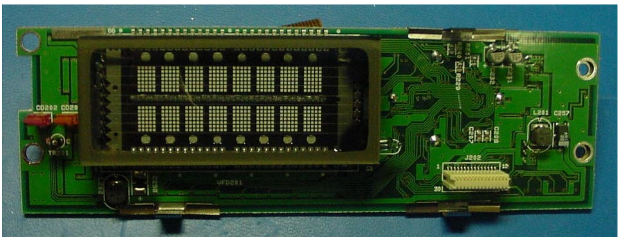
PHOTOGRAPH 30: MAIN BOARD FRONT WITH LCD
