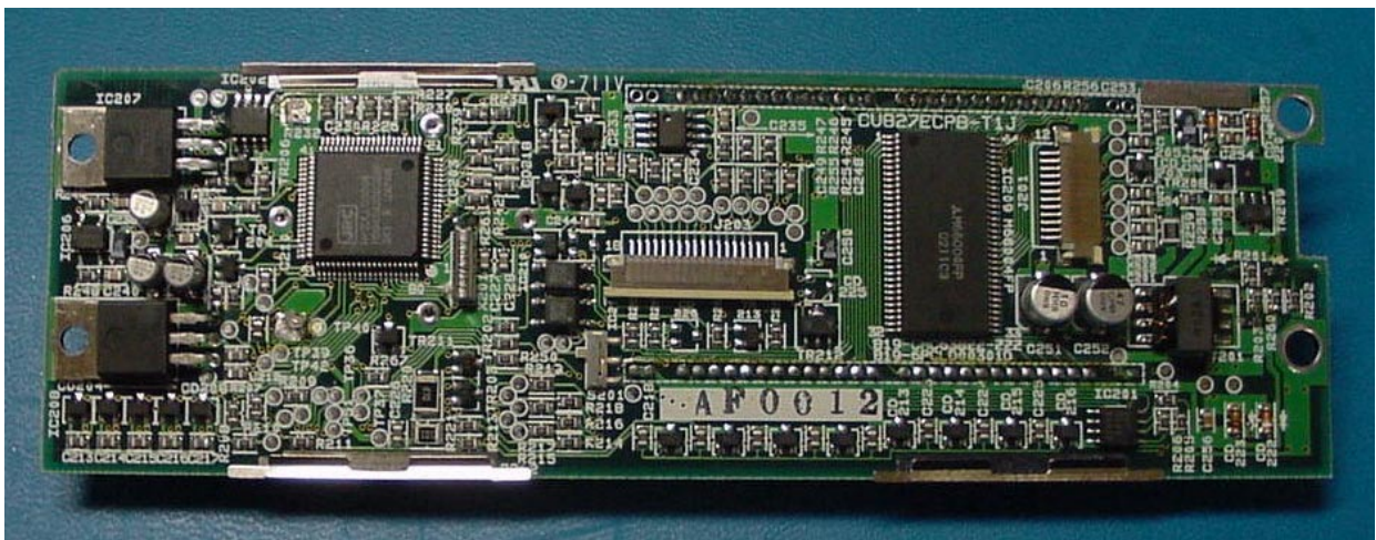
PHOTOGRAPH 32: MAIN BOARD REAR WITHOUT SHIELD
