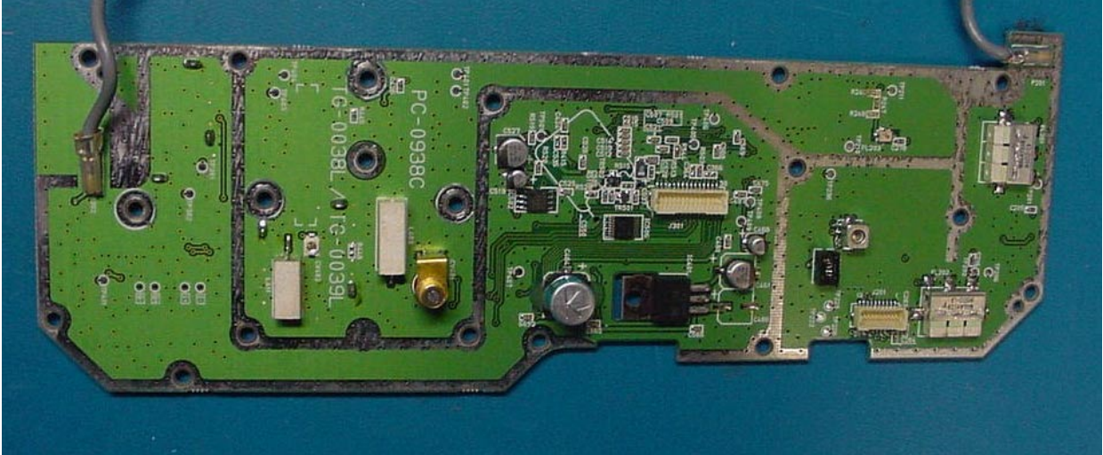
PHOTOGRAPH 14: PCB A FRONT
