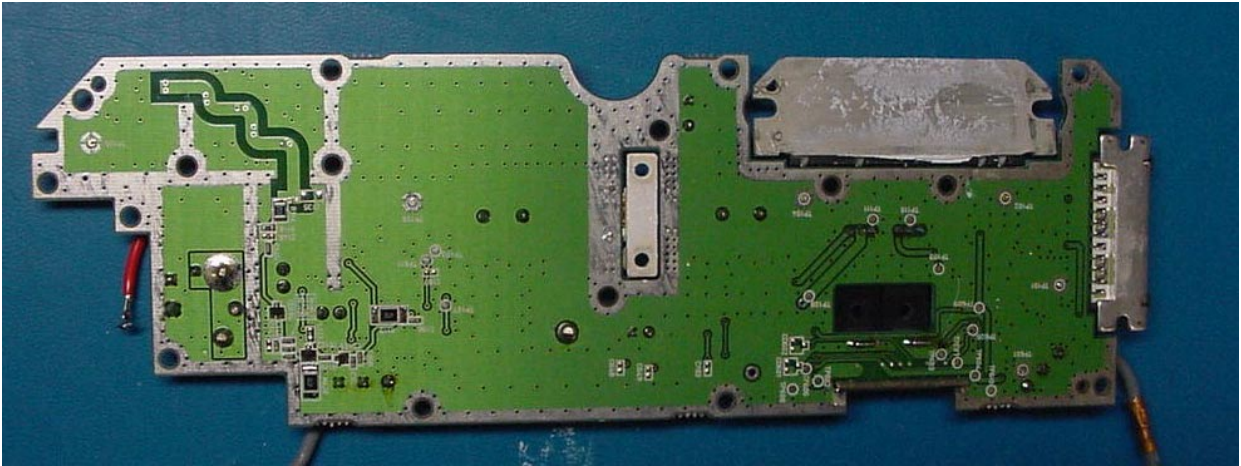
PHOTOGRAPH 18: PCB B REAR
