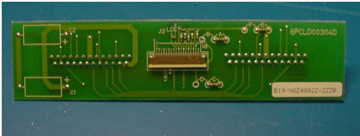
PHOTOGRAPH 38: THIRD BOARD FRONT
