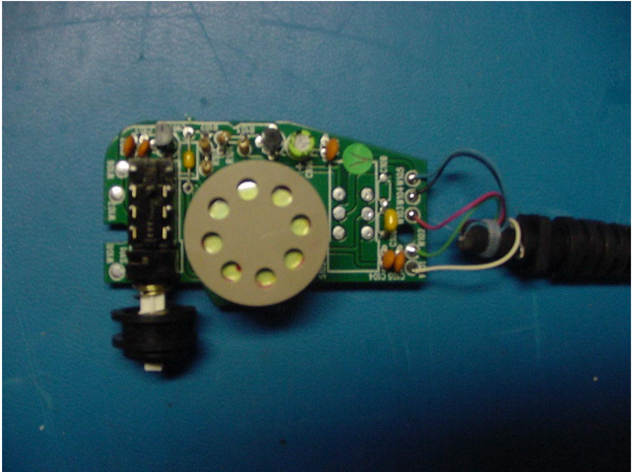
PHOTOGRAPH 24: MIC BOARD FRONT
