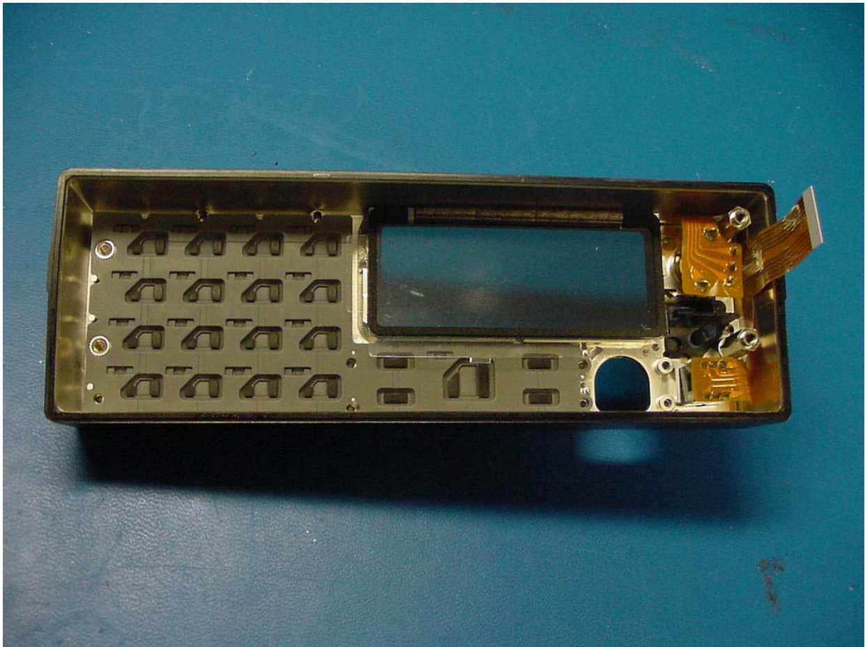
PHOTOGRAPH 29: FRONT COVER INSIDE
