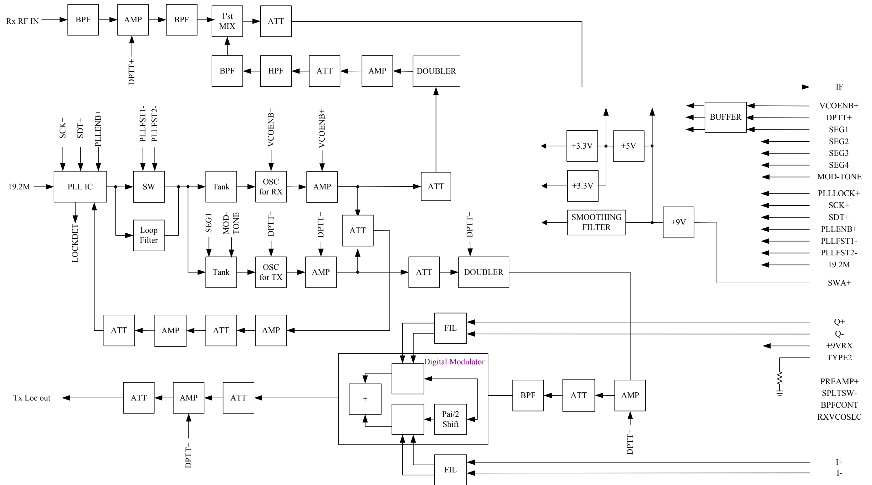
BLOCK DIAGRAM of JAGUAR700M(800MHz) RF/SYNTH Unit TG-0038L
