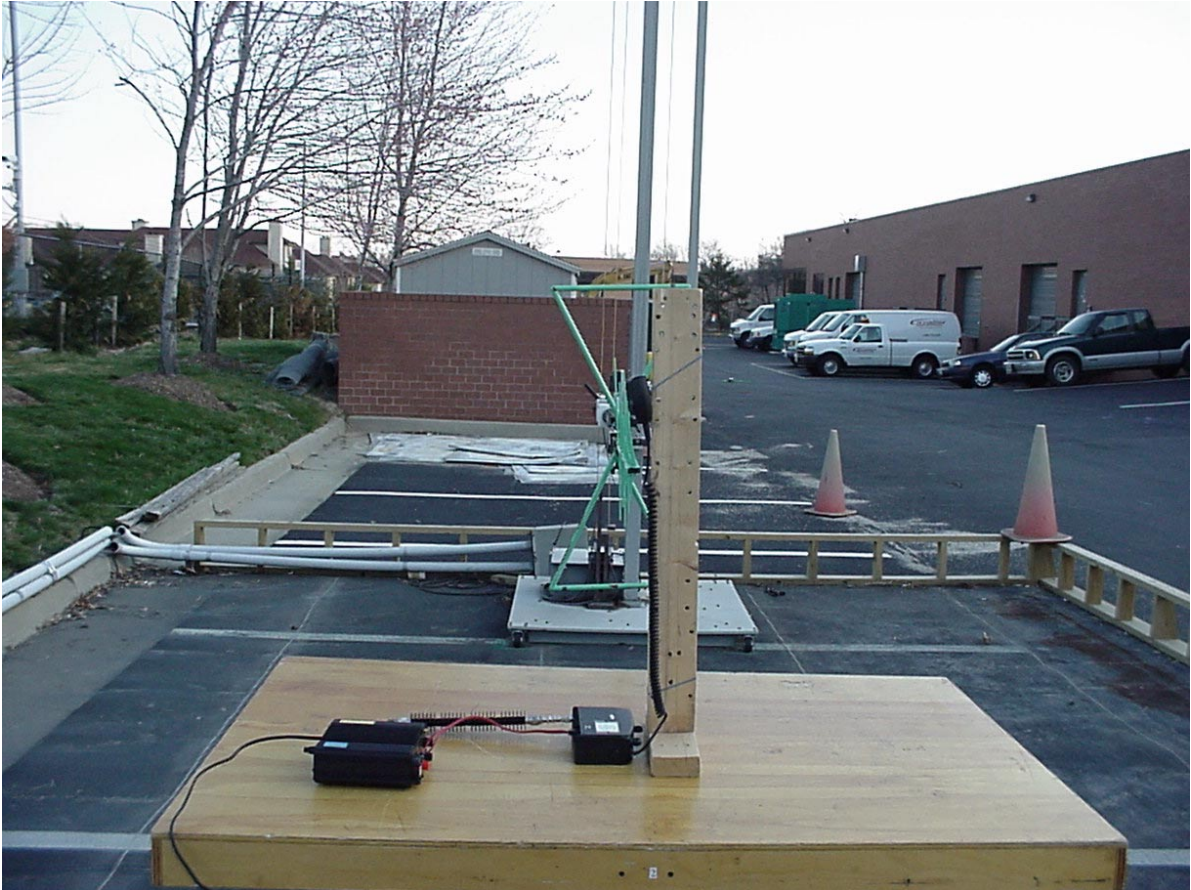
PHOTOGRAPH 1: RADIATED EMISSION TEST FRONT VIEW.
