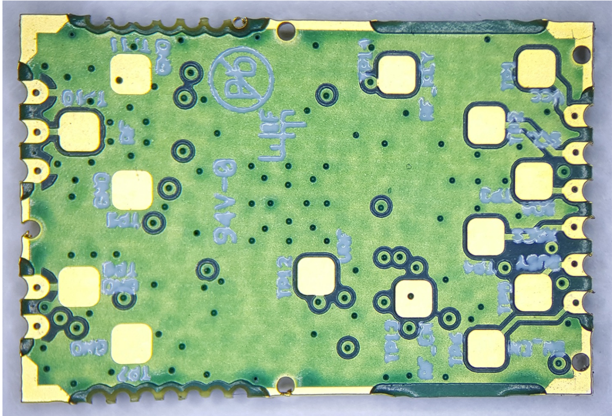
Figure 2. Radio Module, Bottom, without Shield
