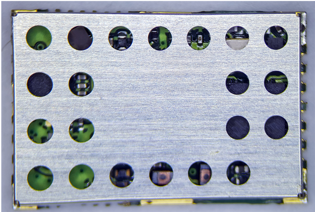
Figure 3. Radio Module with Shield
