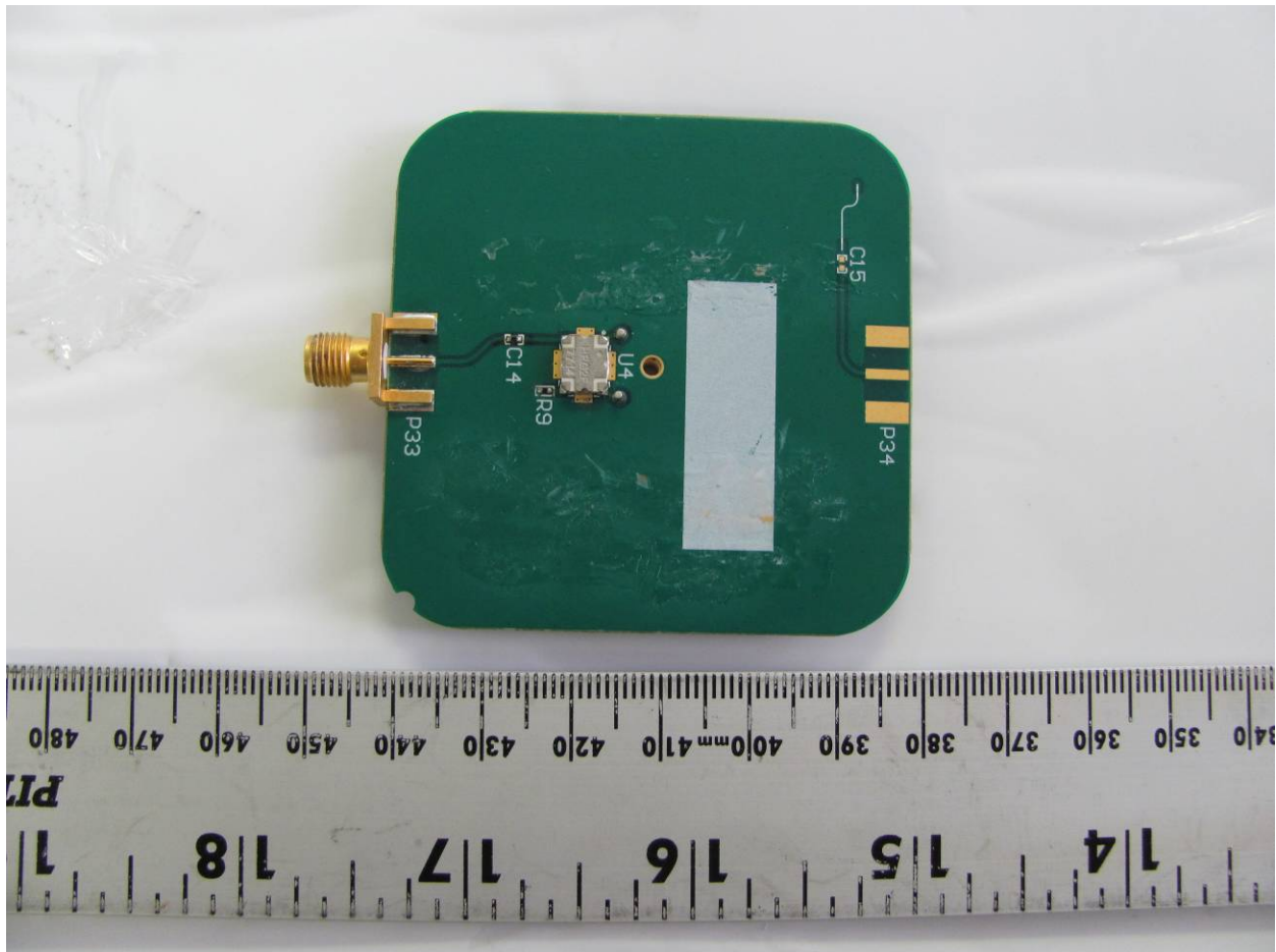
Figure 6. Back of Circular Patch Antenna
