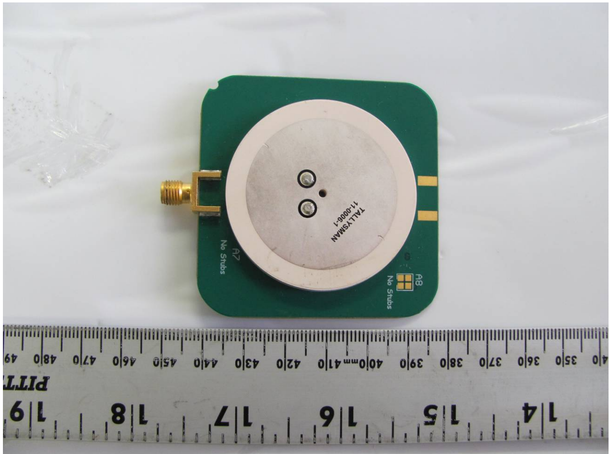
Figure 5. External Circular Patch Antenna
