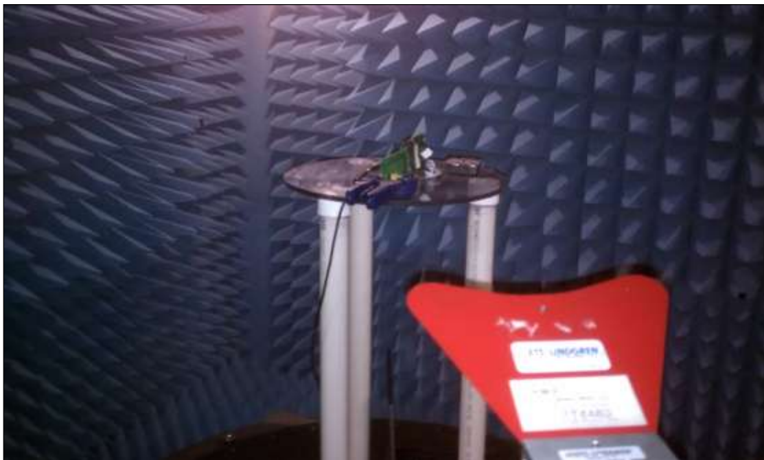
Photograph 3. Radiated Spurious Emissions, HF Test Setup
