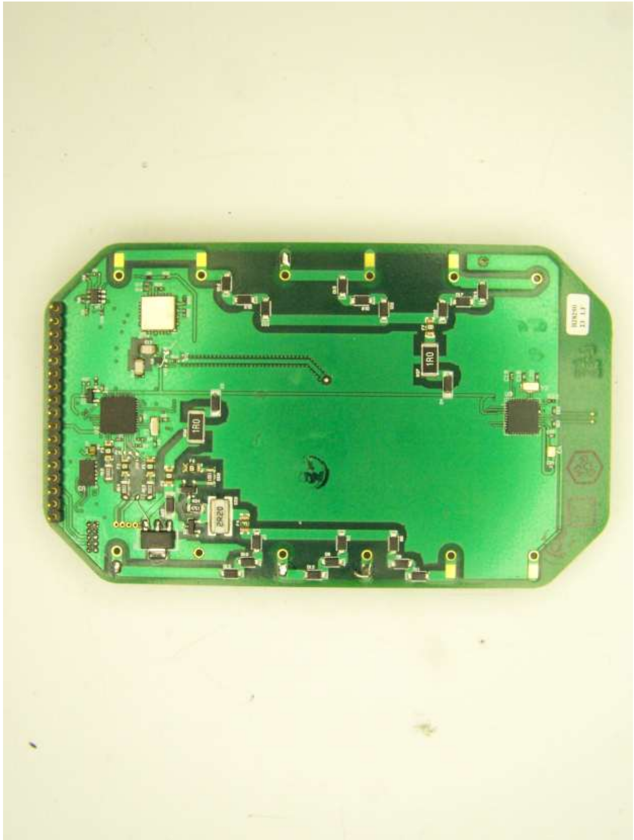
Photograph 3. Board Reverse
