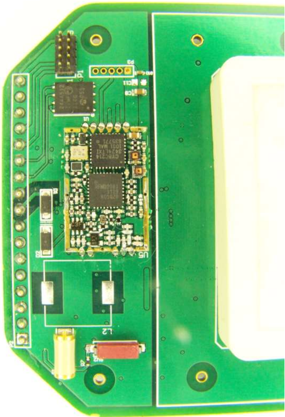
Photograph 4. Components 1
