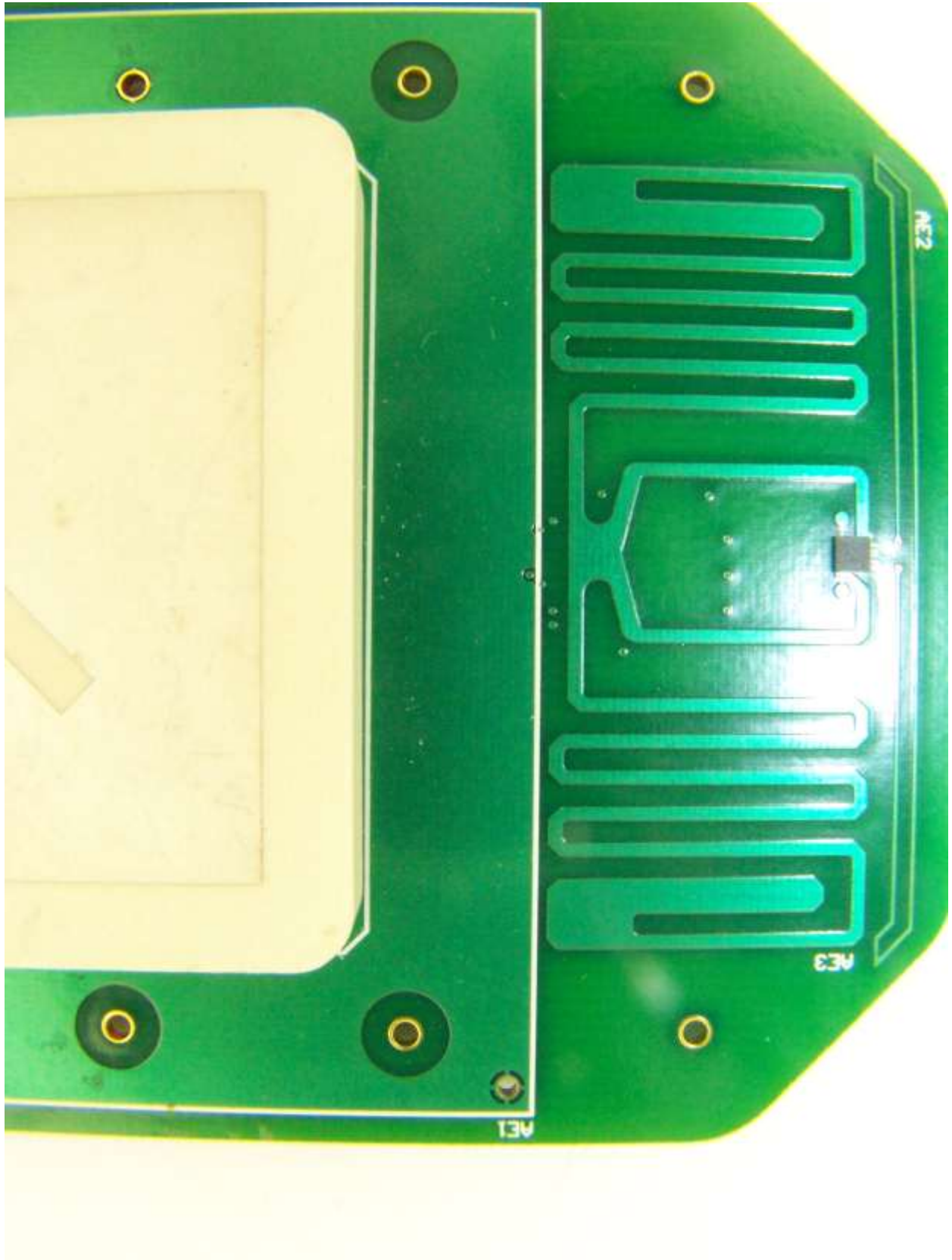
Photograph 5. Components 2
