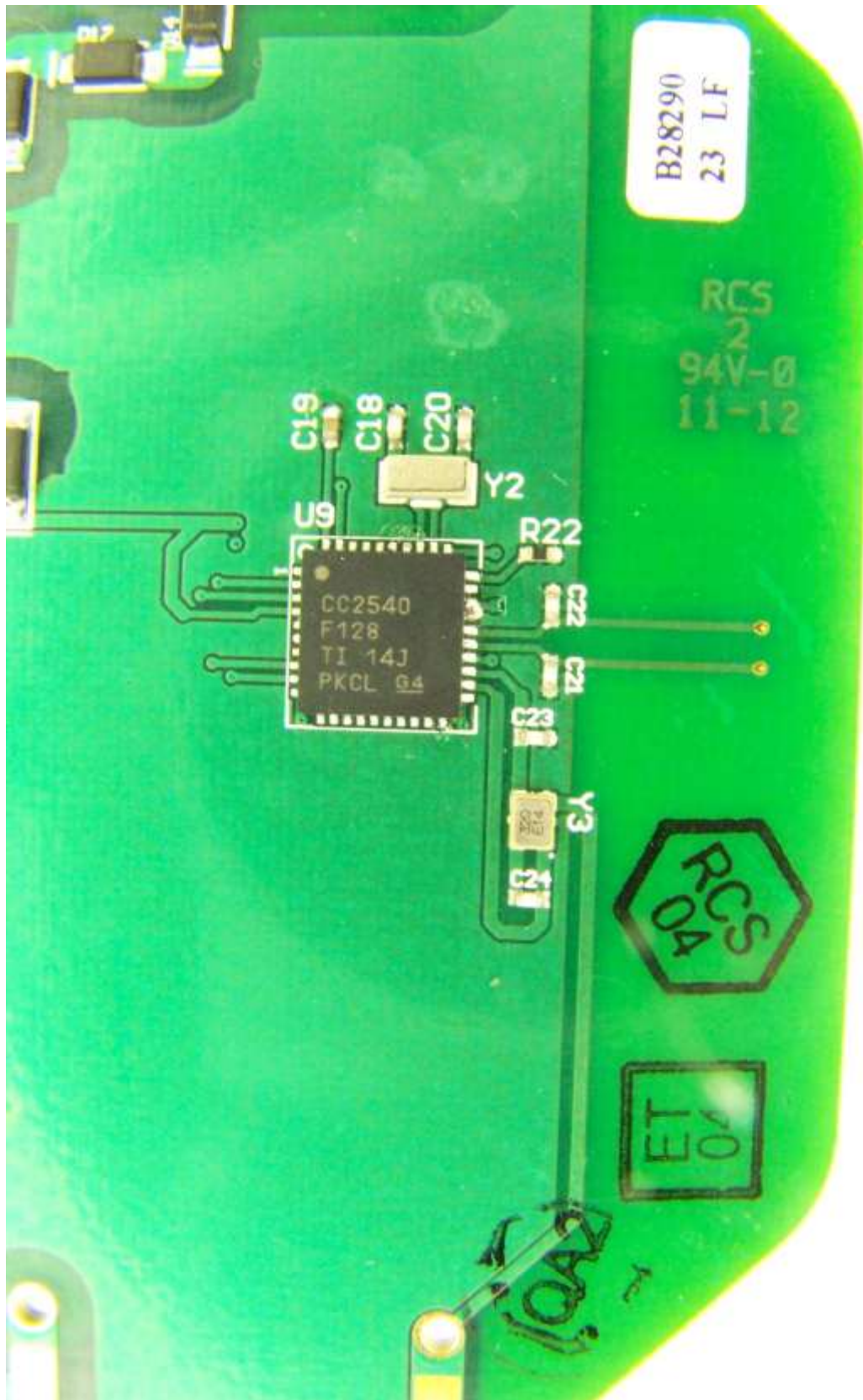
Photograph 8. Components 5
