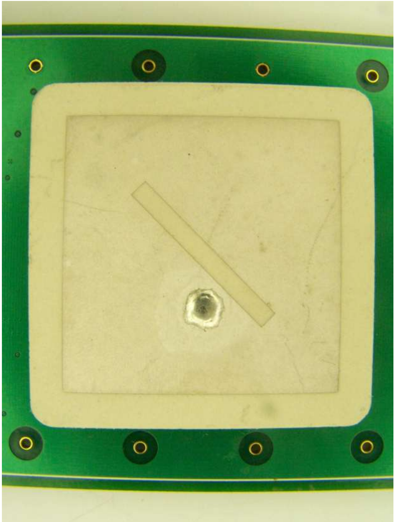
Photograph 1. Antenna
