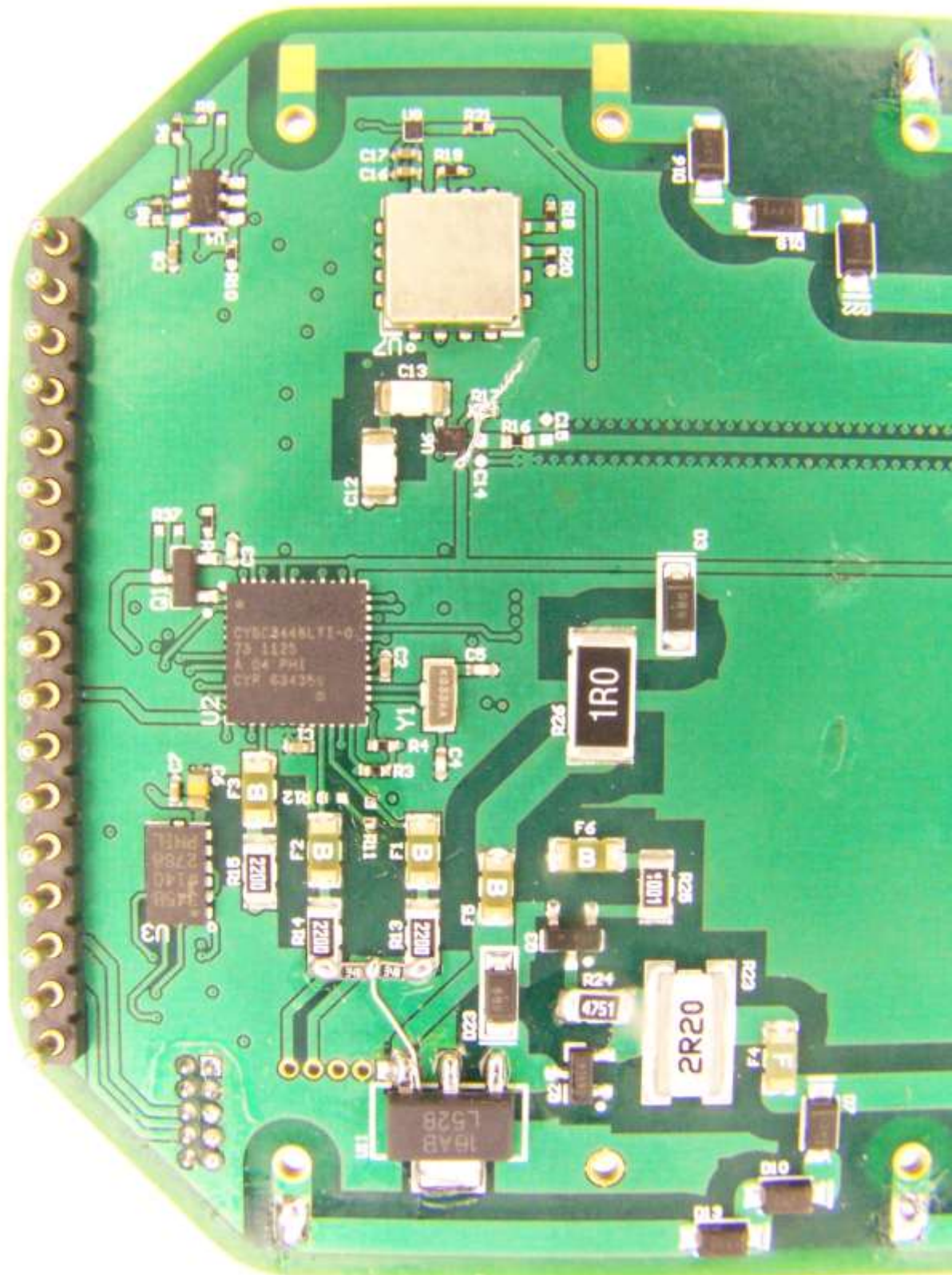
Photograph 6. Components 3
