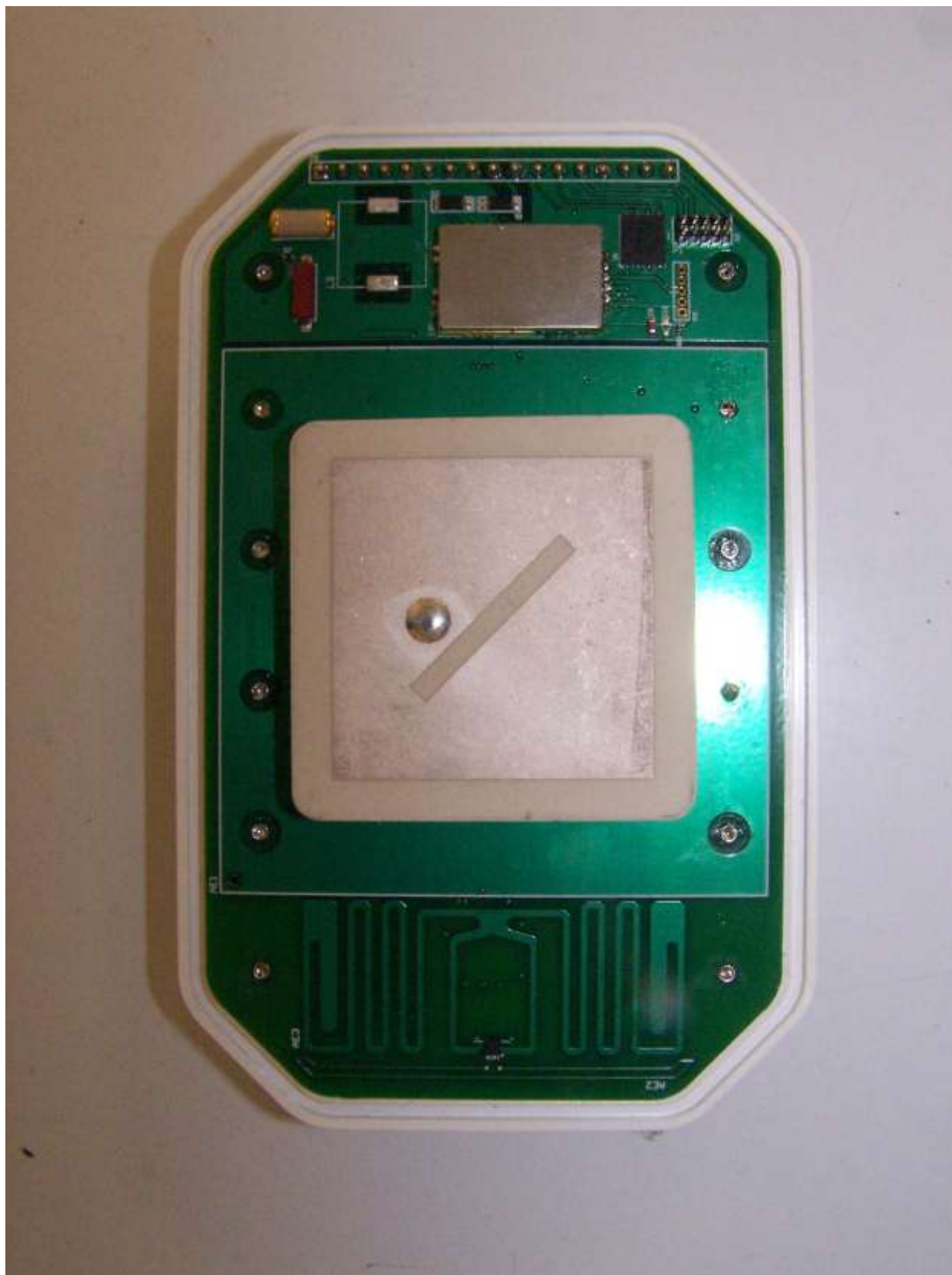
Photograph 2. Board Front
