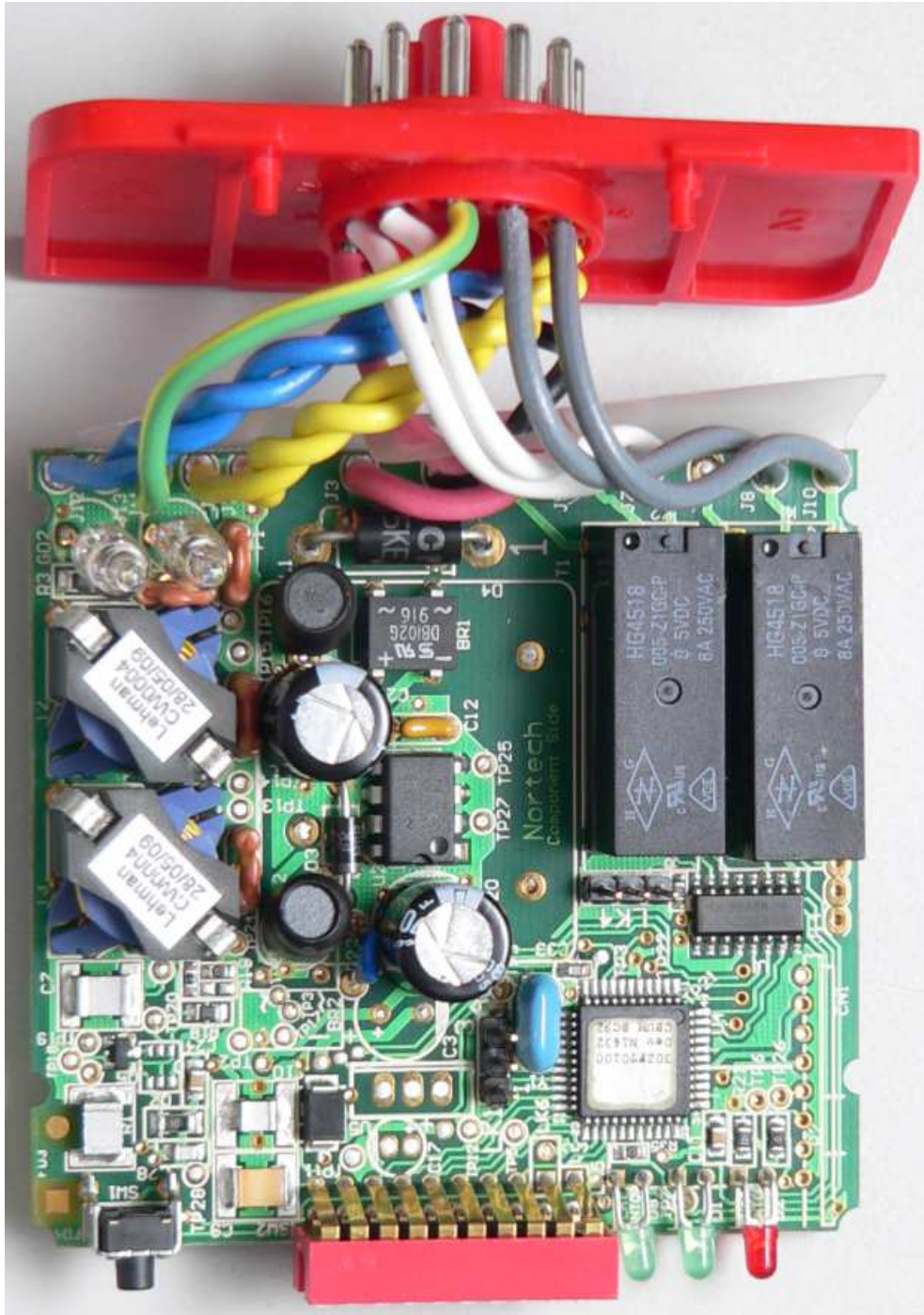
12/24V Models – Interior Top View
