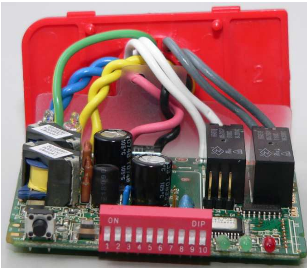
12/24V Models – Interior Front View
