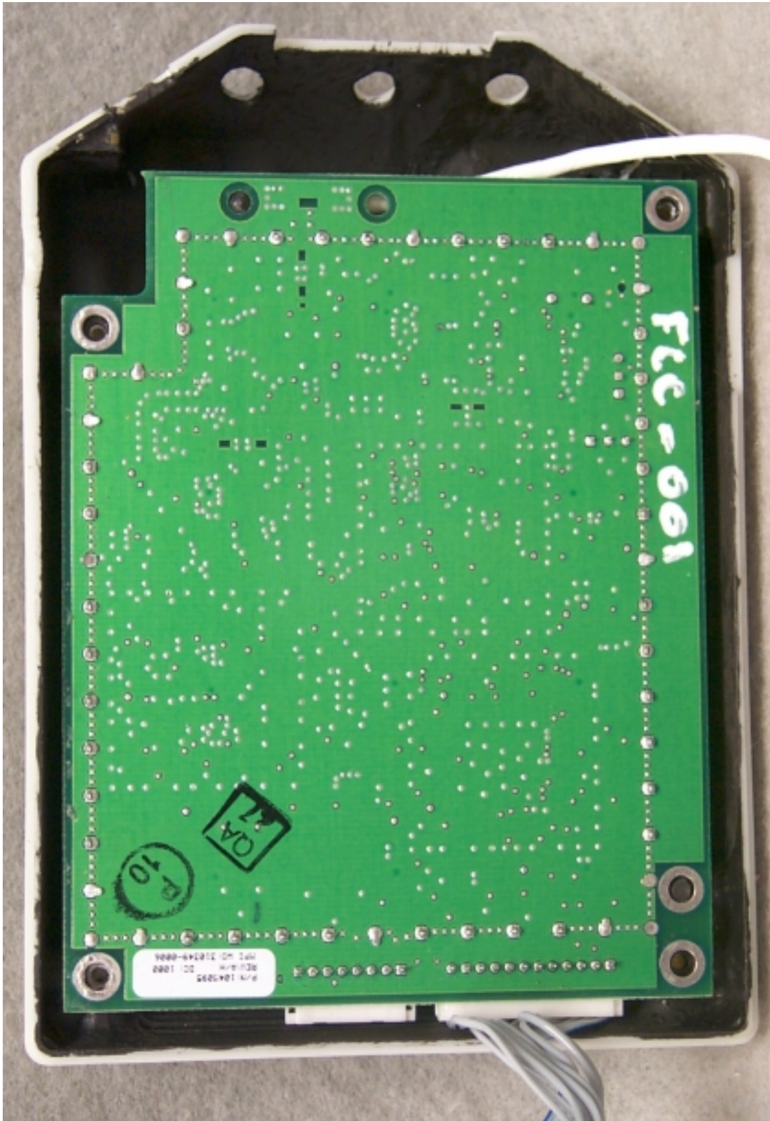
Photo 11. Bottom View of Transceiver Board
