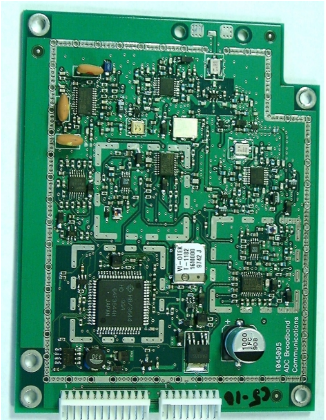
Photo 10. Top View of Transceiver Board, Sub Shields Removed
