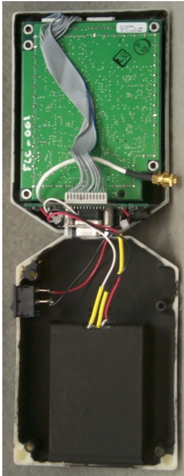
Photo 5. Internal View of EUT, Housing Opened
