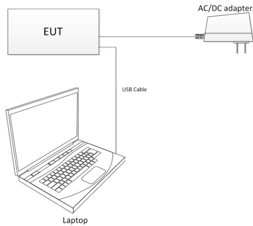
Figure 3.6-1: Setup diagram
