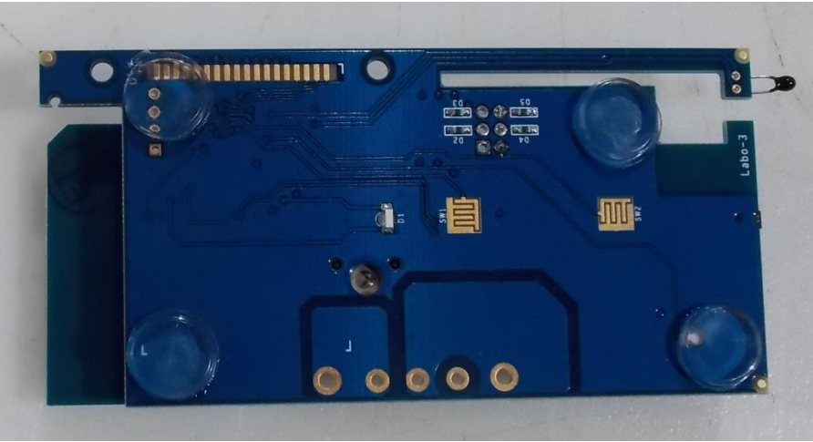
Figure 10.1-2: Bottom view
