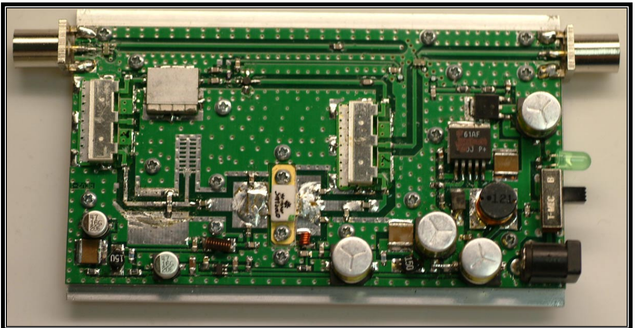
PHOTOGRAPH 13: PCB TOP VIEW
