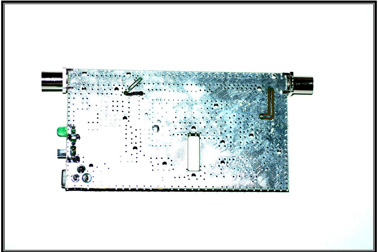
PHOTOGRAPH 14: BOTTOM OF AMP PCB WITHOUT SHIELDS
