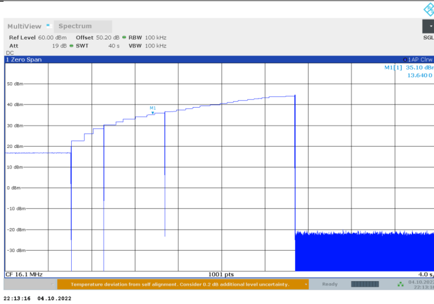
Figure 8.2-1: Modulation Characteristic Modulation limiting
