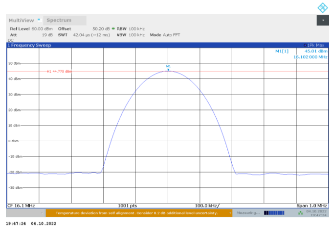
Figure 8.1-2: Mid channel, 16.1 MHz, 30W, J3E modulation, output power
