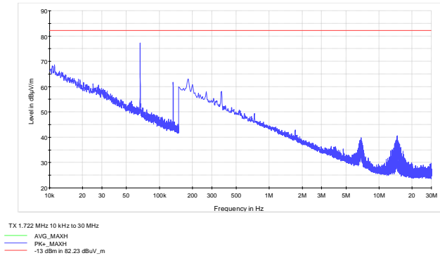
Figure 8.5-1: Low channel Radiated Spurious
