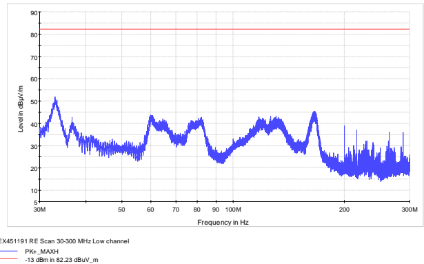
Figure 8.5-2: Low channel Radiated Spurious
