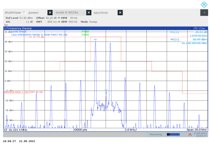
Figure 8.3-2: Mid channel Mask 30W 400 Hz and 1800 Hz
