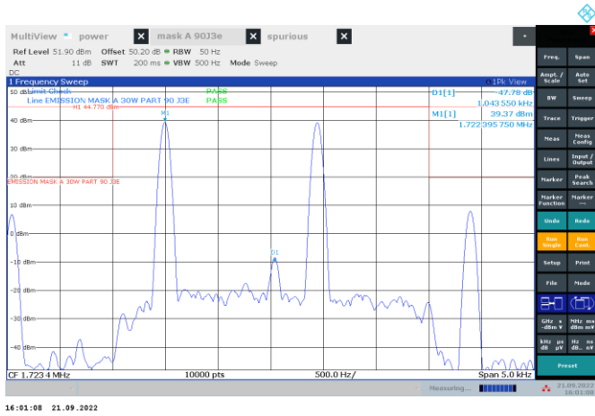
Figure 8.3-7: Low channel 30W 400 Hz and 1800 Hz 40 dB Carrier suppression
