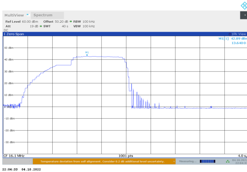
Figure 8.2-2: Modulation Characteristic Audio Frequency Response
