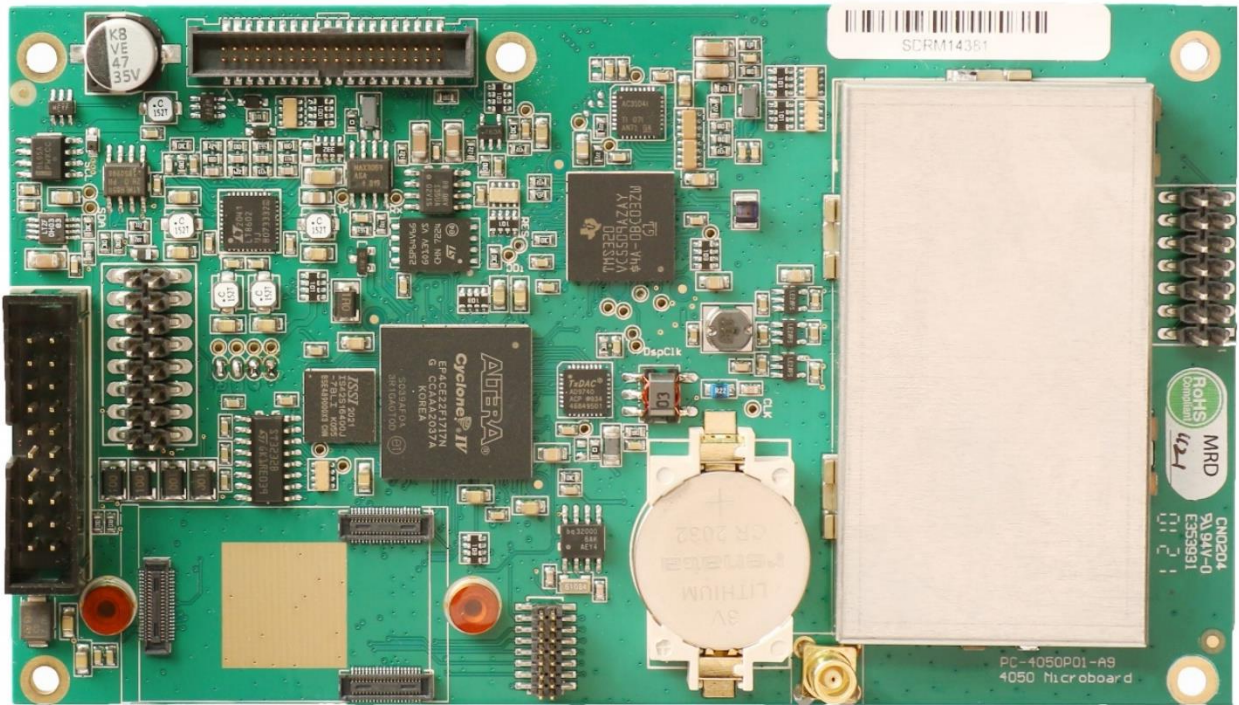
PRC-4090 Transceiver – Micro board (top view)
