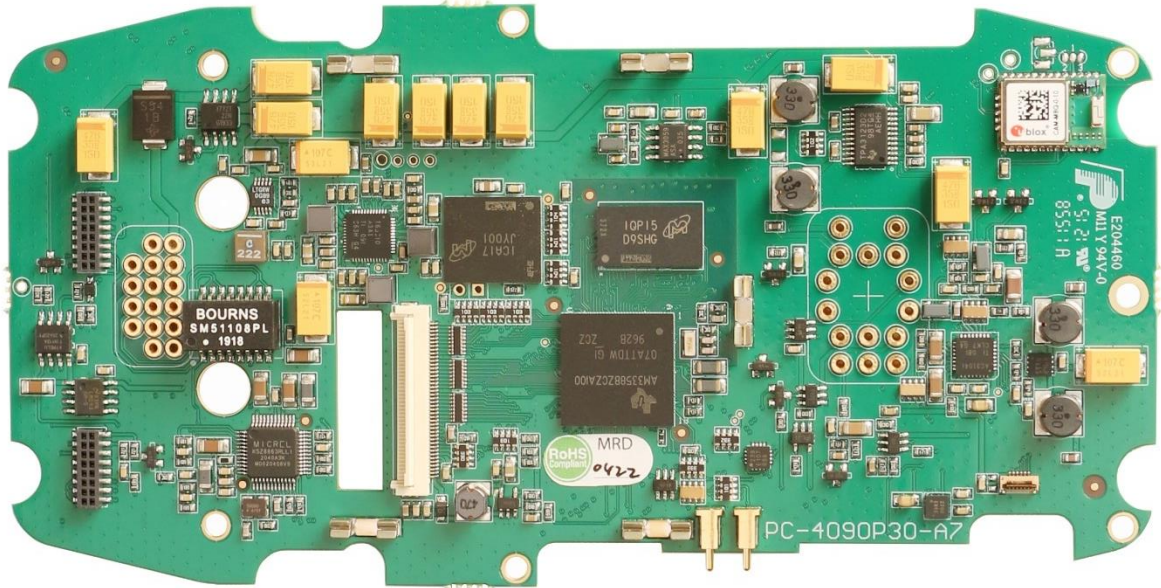
PRC-4090 Handset board - (top view)
