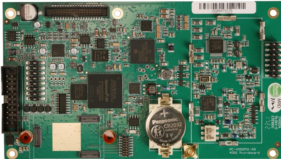
PRC-4090 Transceiver - Micro board (top view without RF shield)
