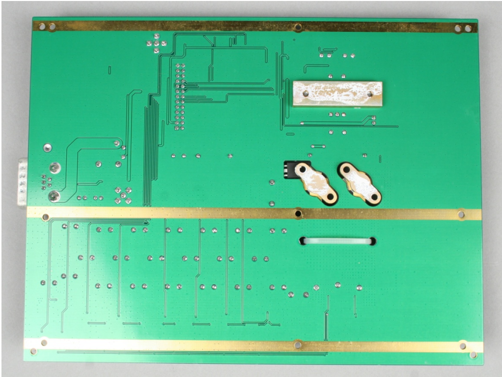
PRC-2090 PA PCB, Bottom View SA-02010
