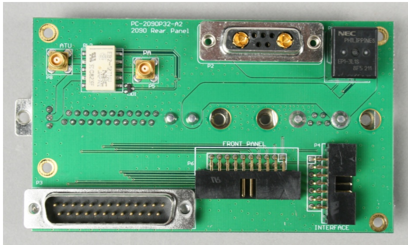
Rear Panel PCB, Top View
