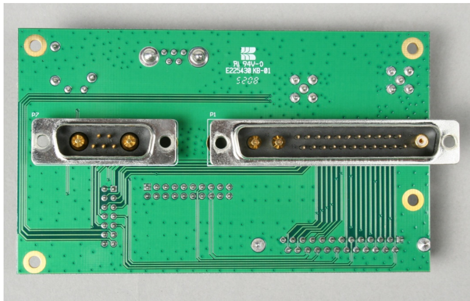
Rear Panel PCB, Bottom View
