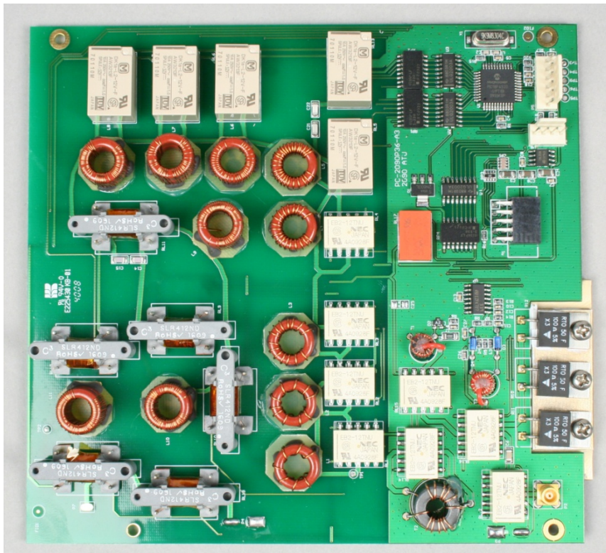
PRC-2090 ATU PCB, Top View SA-20936
