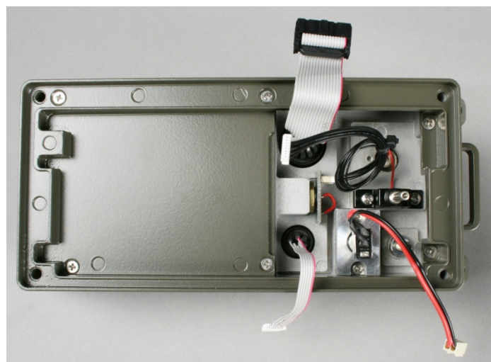
PRC-2090 Front Panel, Internal View
