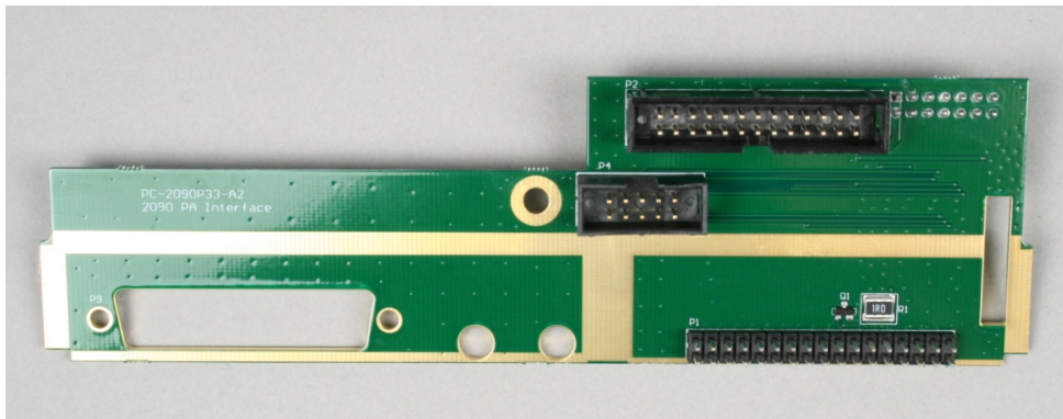
PRC-2090 PA Interface PCB, Top View SA-20933
