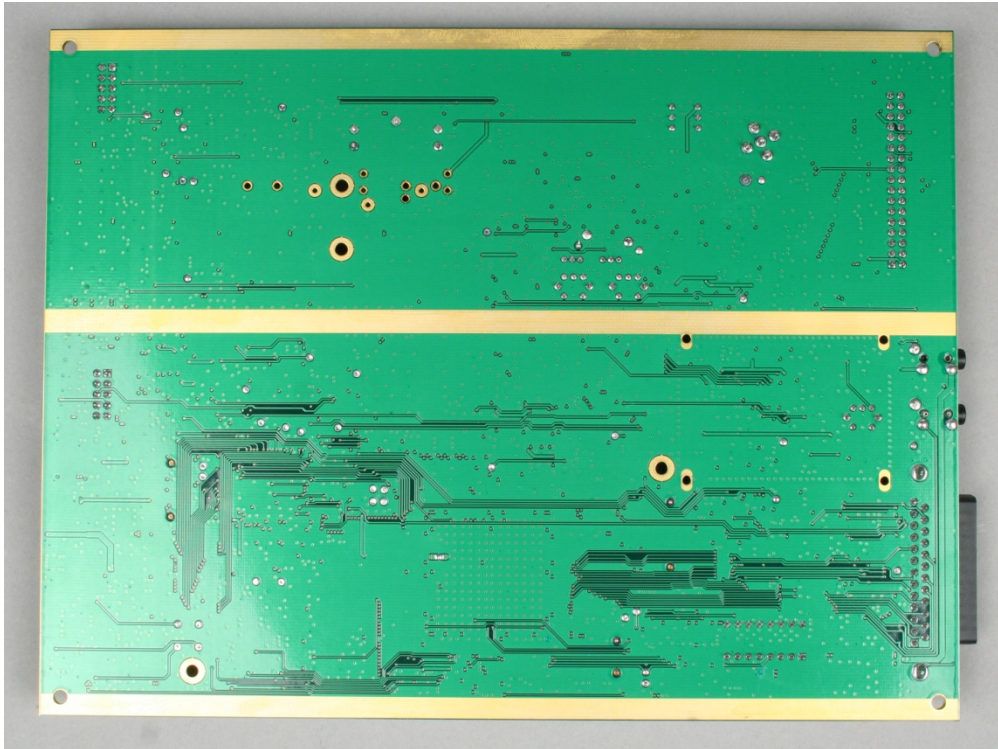
PRC-2090 Microprocessor/RF/Audio PCB, Bottom View SA-02000
