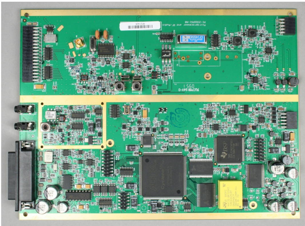
PRC-2090 Microprocessor/RF/Audio PCB, Top View SA-02000
