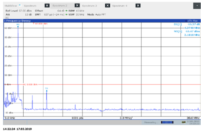
Figure 8.5-4: Low channel Conducted Spurious 1000W J3E
