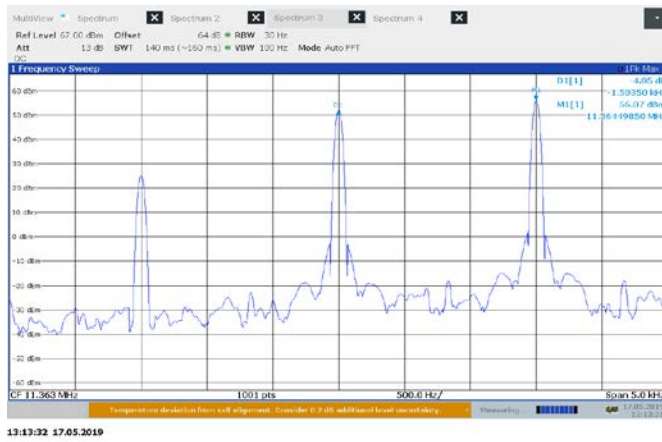
Figure 8.4-5: Mid channel 1000W H3E 6 dB
