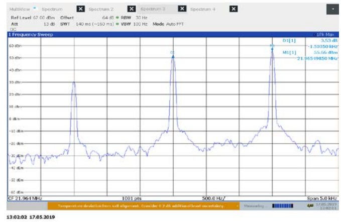
Figure 8.4-6: High channel 1000W H3E 6 dB
