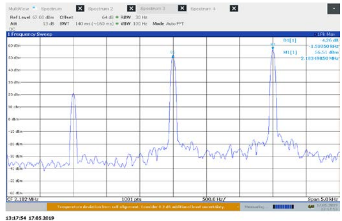
Figure 8.4-4: Low channel 1000W H3E 6 dB
