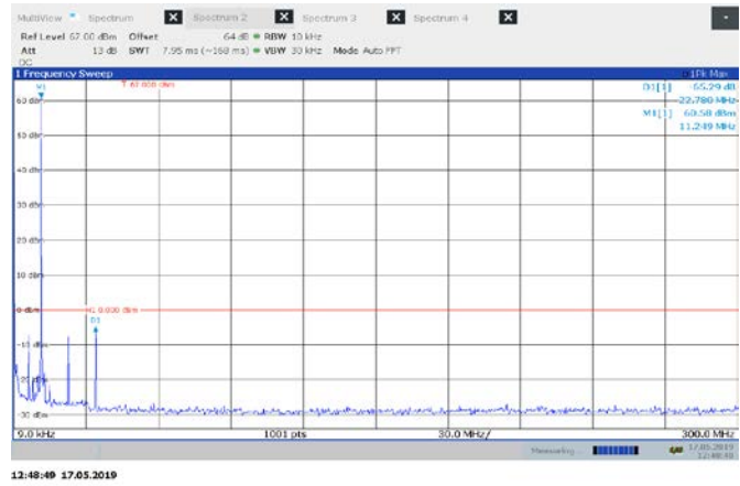
Figure 8.5-2: Mid channel Conducted Spurious 1000W H3E
