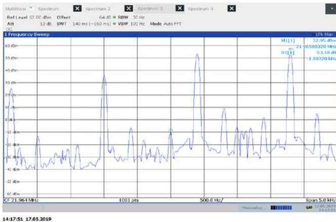
Figure 8.4-3: High channel 1000W J3E 40 dB
