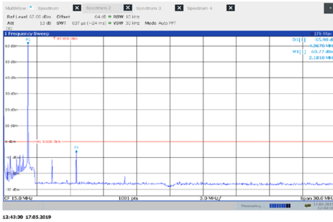
Figure 8.5-1: Low channel Conducted Spurious 1000W H3E
