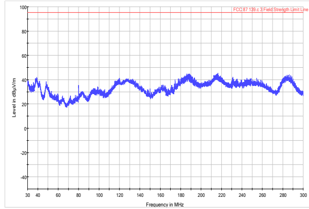
Low channel 1000 W 400 Hz and 1800 Hz PK+ MAXH [Result Table Result:1] FCC 87.139.c.3 Field Strength Limit Line [..EMI Radiated/Wireless Limits]
