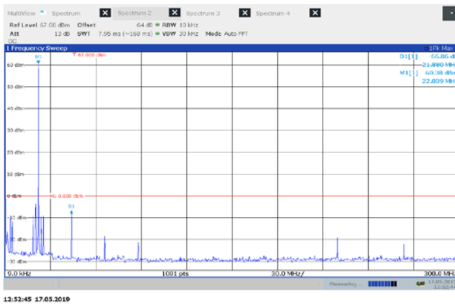
Figure 8.5-3: High channel Conducted Spurious 1000W H3E
