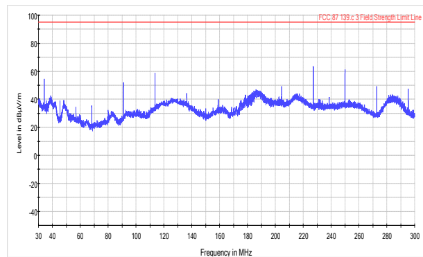
Mid channel 1000 W 400 Hz and 1800 Hz PK+ MAXH FCC 87.139.c.3 Field Strength Limit Line
