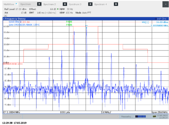
Figure 8.3-4: Low channel Mask 1000W H3E
