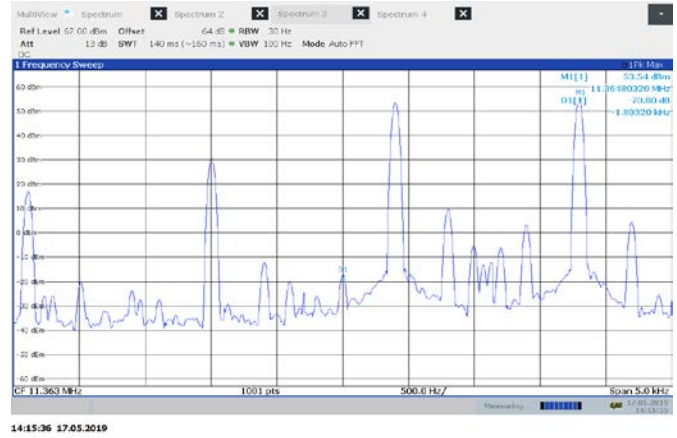
Figure 8.4-2: Mid channel 1000W J3E 40 dB
