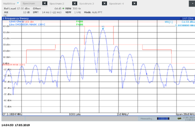
Figure 8.3-1: Low channel Mask 1000W J3E
