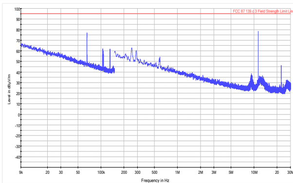
mid channel 1000 W 9 kHz-30 MHz spurious emission PK+ MAXH FCC 87.139.c.3 Field Strength Limit Line
