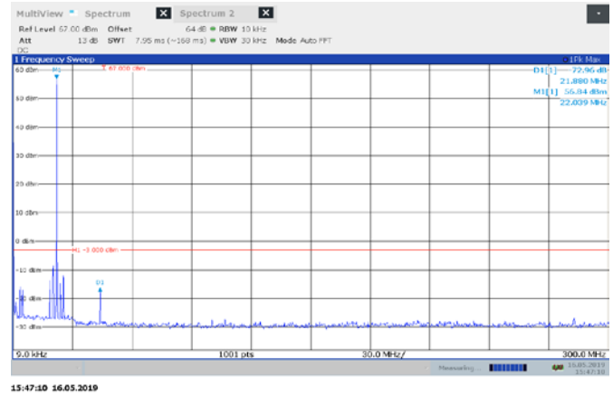
Figure 8.5-6: High channel Conducted Spurious 100W J3E
