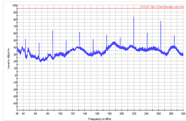
High channel 1000 W 400 Hz and 1800 Hz PK+ MAXH FCC 87.139.c.3 Field Strength Limit Line
