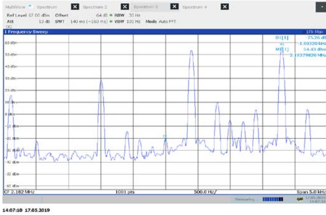
Figure 8.4-1: Low channel 1000W J3E 40 dB
