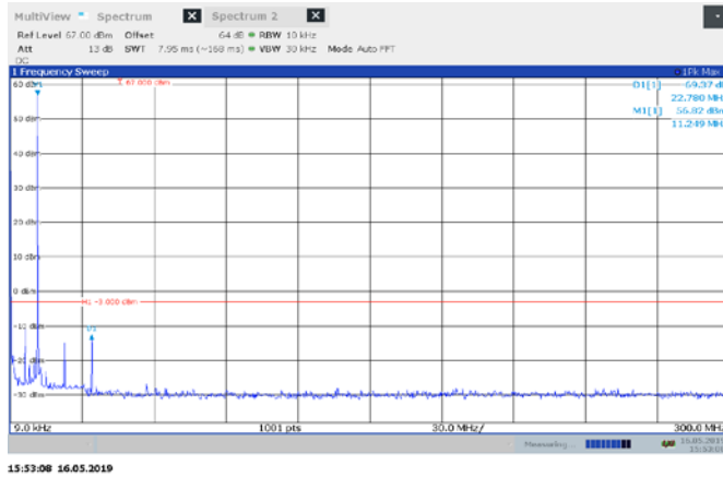
Figure 8.5-5: Mid channel Conducted Spurious 100W J3E
