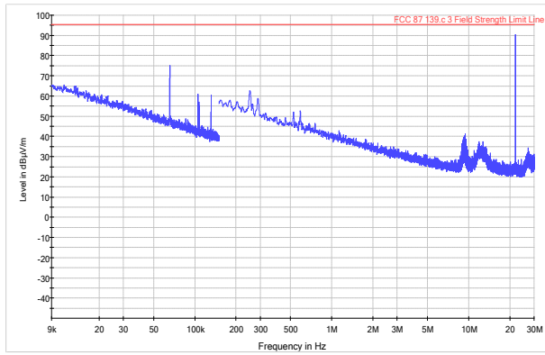
high channel 1000 W 9 kHz-30 MHz spurious emission PK+ MAXH FCC 87.139.c.3 Field Strength Limit Line
