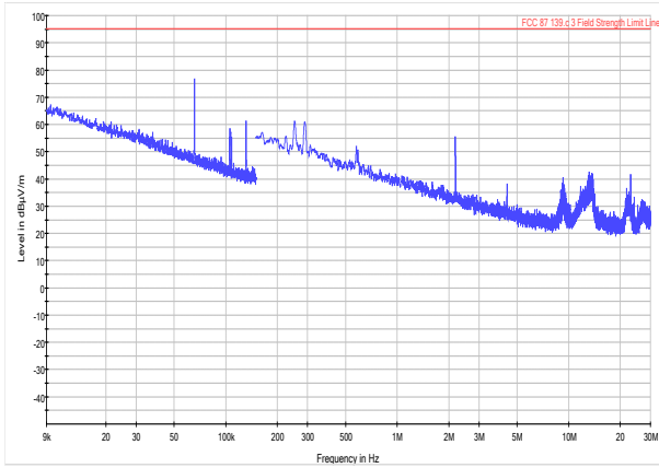
low channel 1000 W 9 kHz-30 MHz spurious emission PK+ MAXH FCC 87.139.c.3 Field Strength Limit Line
