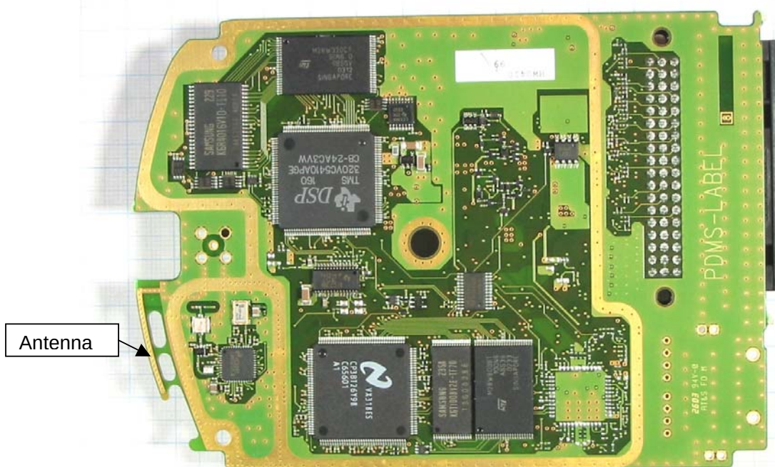
Figure 1: Top view of PWB
