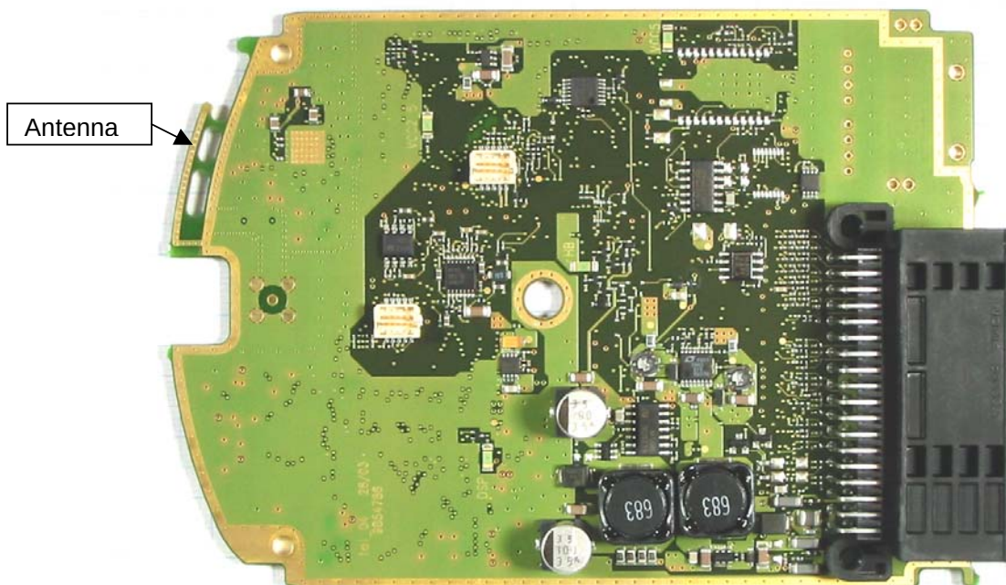
Figure 1: Top view of PWB
