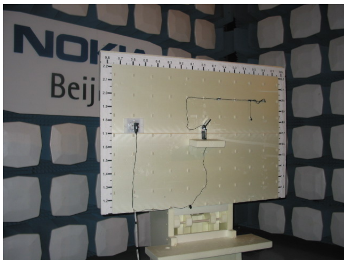
Picture 1 Radiated RF output power measurement – flip opened
