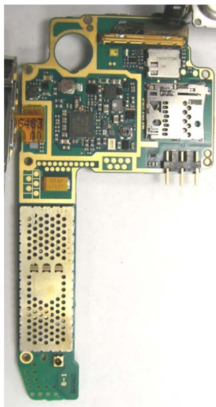
PWB with shielding
