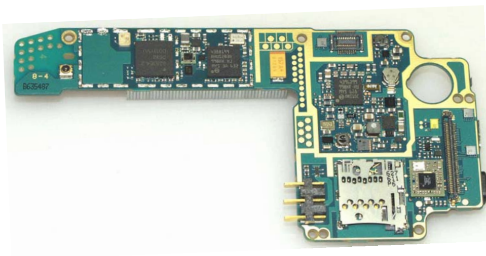
PWB without shielding
