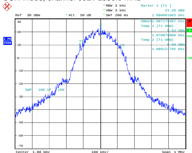
GSM mode, channel 661 / 1880.0 MHz
