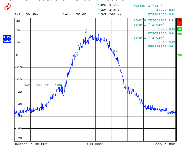
EGPRS mode, channel 661 / 1880.0 MHz
