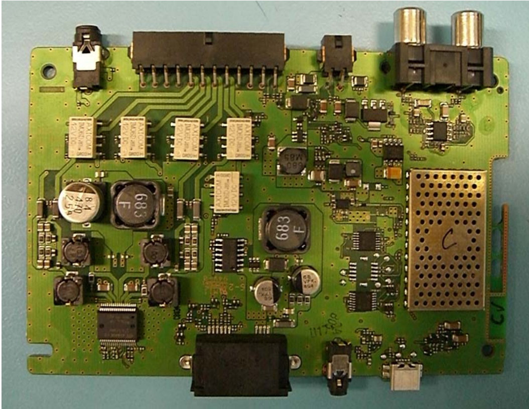
PWB bottom view
