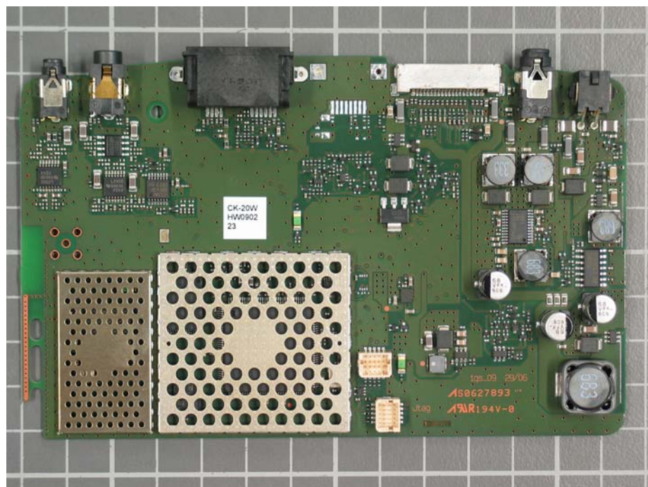
Top view of PWB with shielding
