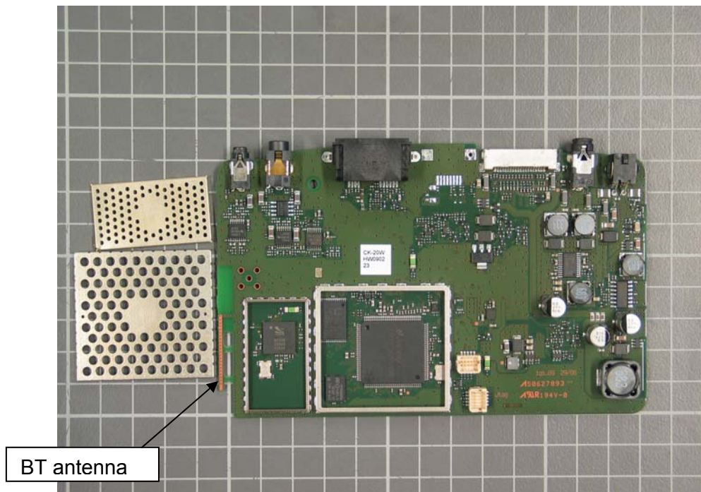
Top view of PWB without shielding
