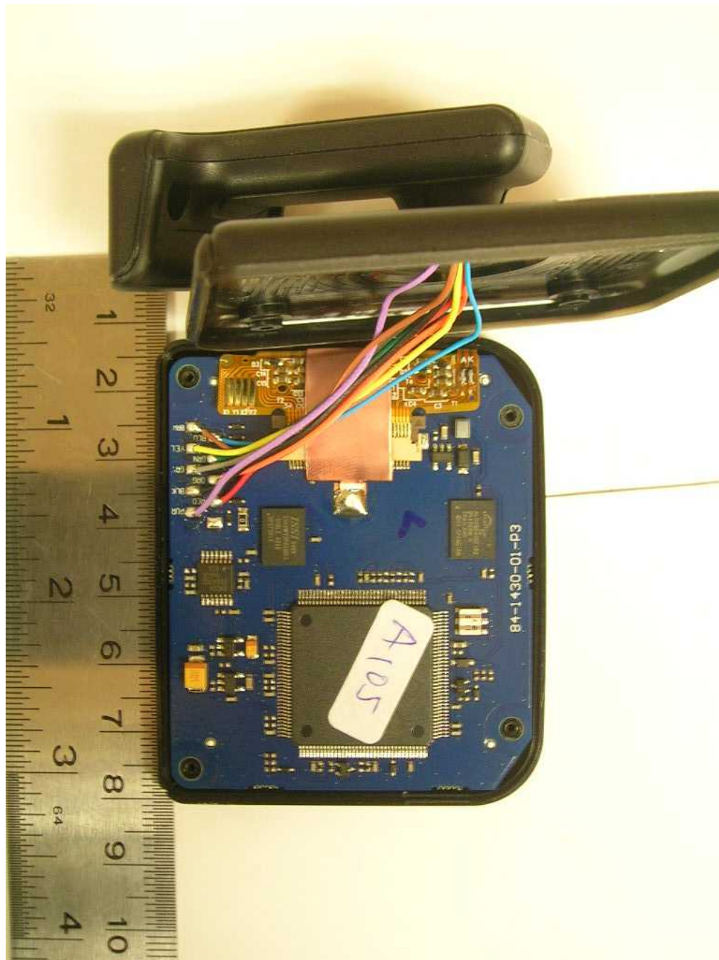
LCD Board – Internal View
