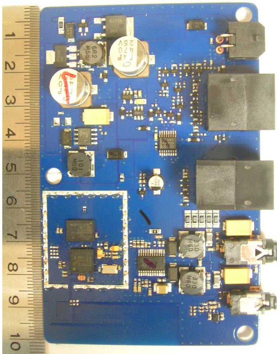
Main Unit Board - Component Side
