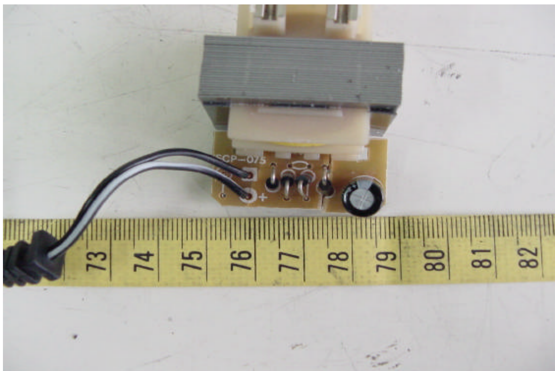
Component View of Adapter's PCB
