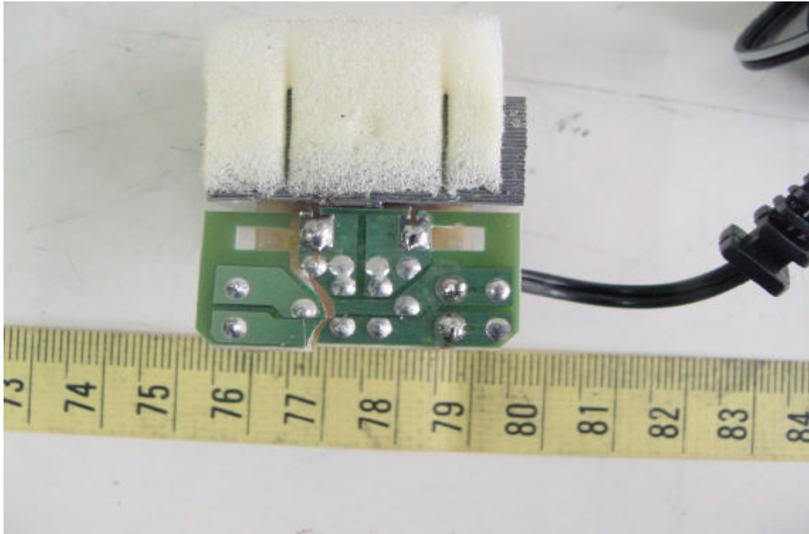
Solder View of Adapter's PCB
