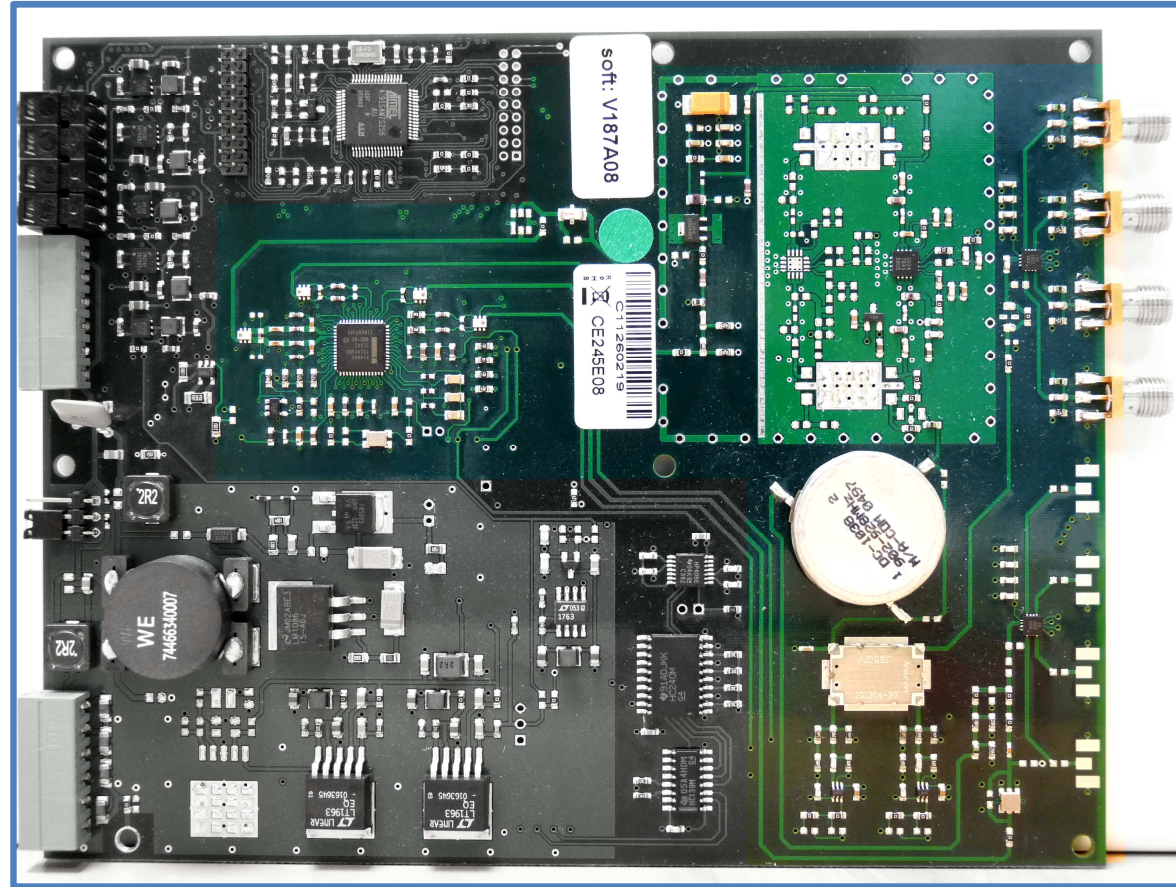
RFID board without EMI Shield (RF blocks are colored)
