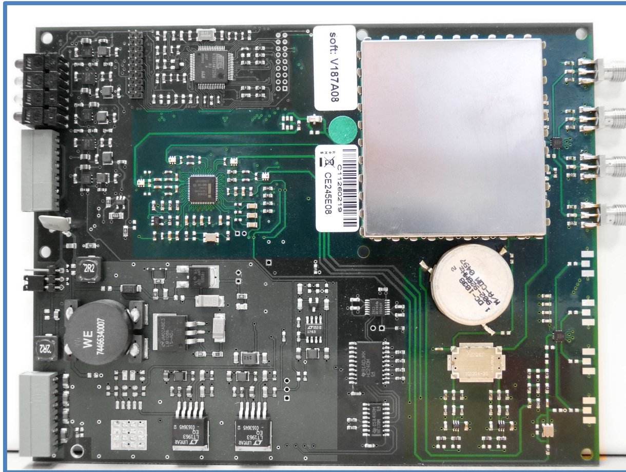
RFID board With EMI Shield (RF blocks are colored)
