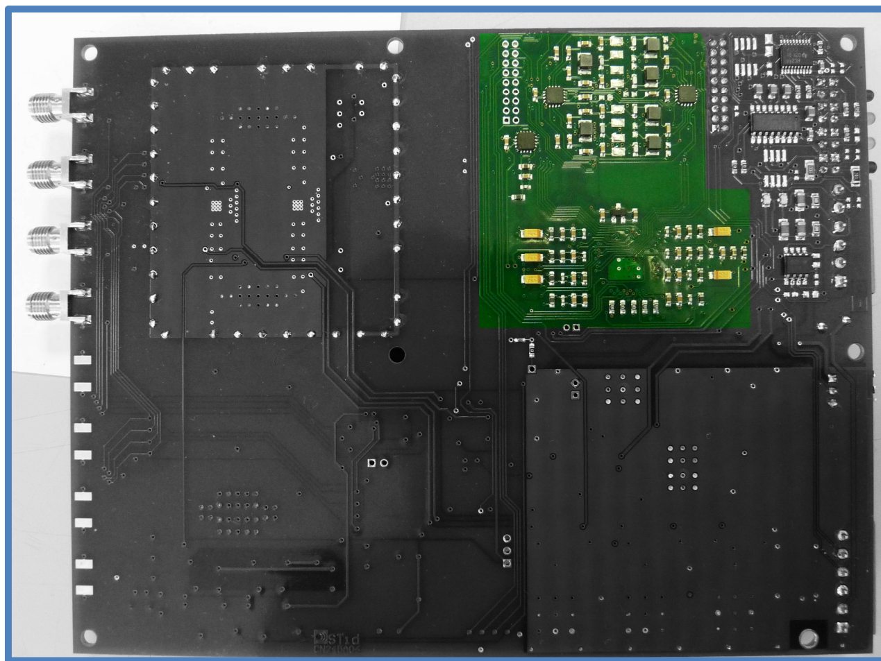
RFID board solder side (RF blocks are colored). No EMI shield is mounted
