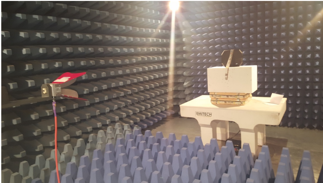
TEST SETUP PHOTO(S) - F>1GHz
