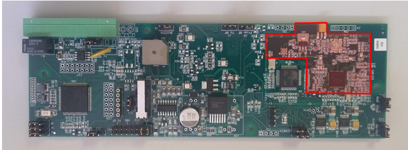
RFID BOARD TOP SIDE WITHOUT EMI SHIELD (RF block is colored)
