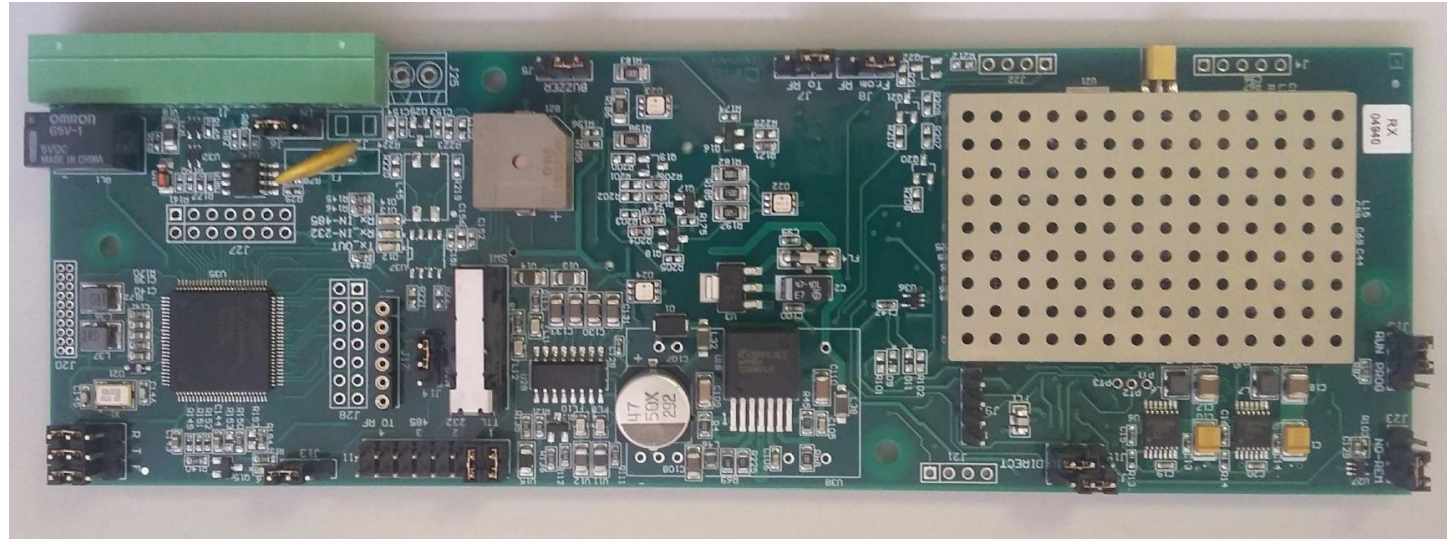
RFID BOARD TOP SIDE WITH EMI SHIELD
