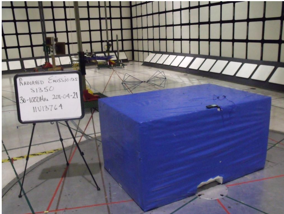
Figure 6 Test setup for Radiated Emissions – Battery Powered
