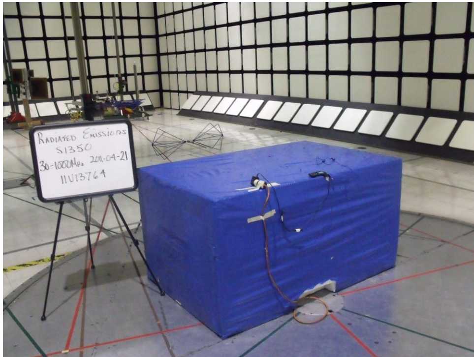
Figure 5 Test setup for Radiated Emissions – AC Powered
