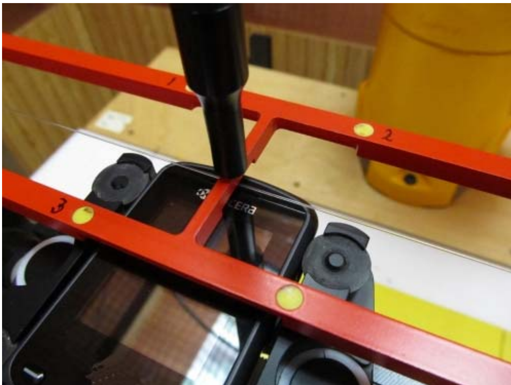
Figure 1b – HAC RF Emission Test Setup
