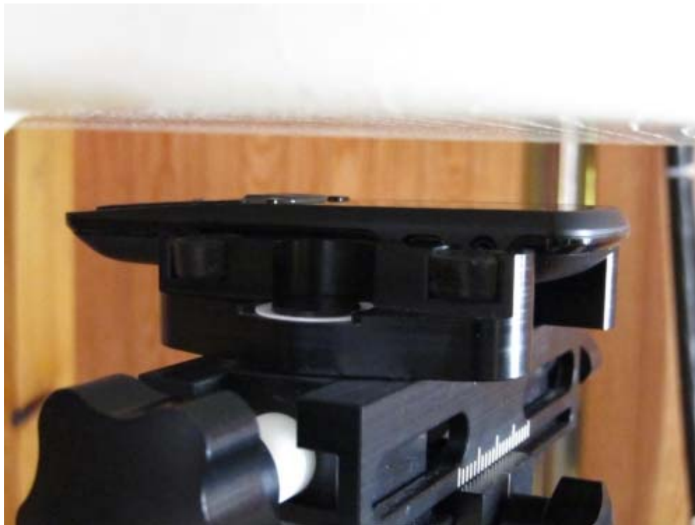
Figure 9E.4 Body SAR setup (Face Up, 15mm Air Separation)
