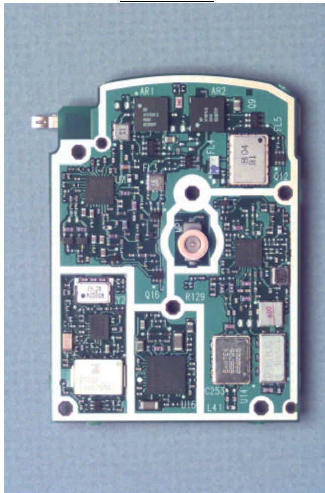
RF Module Front
